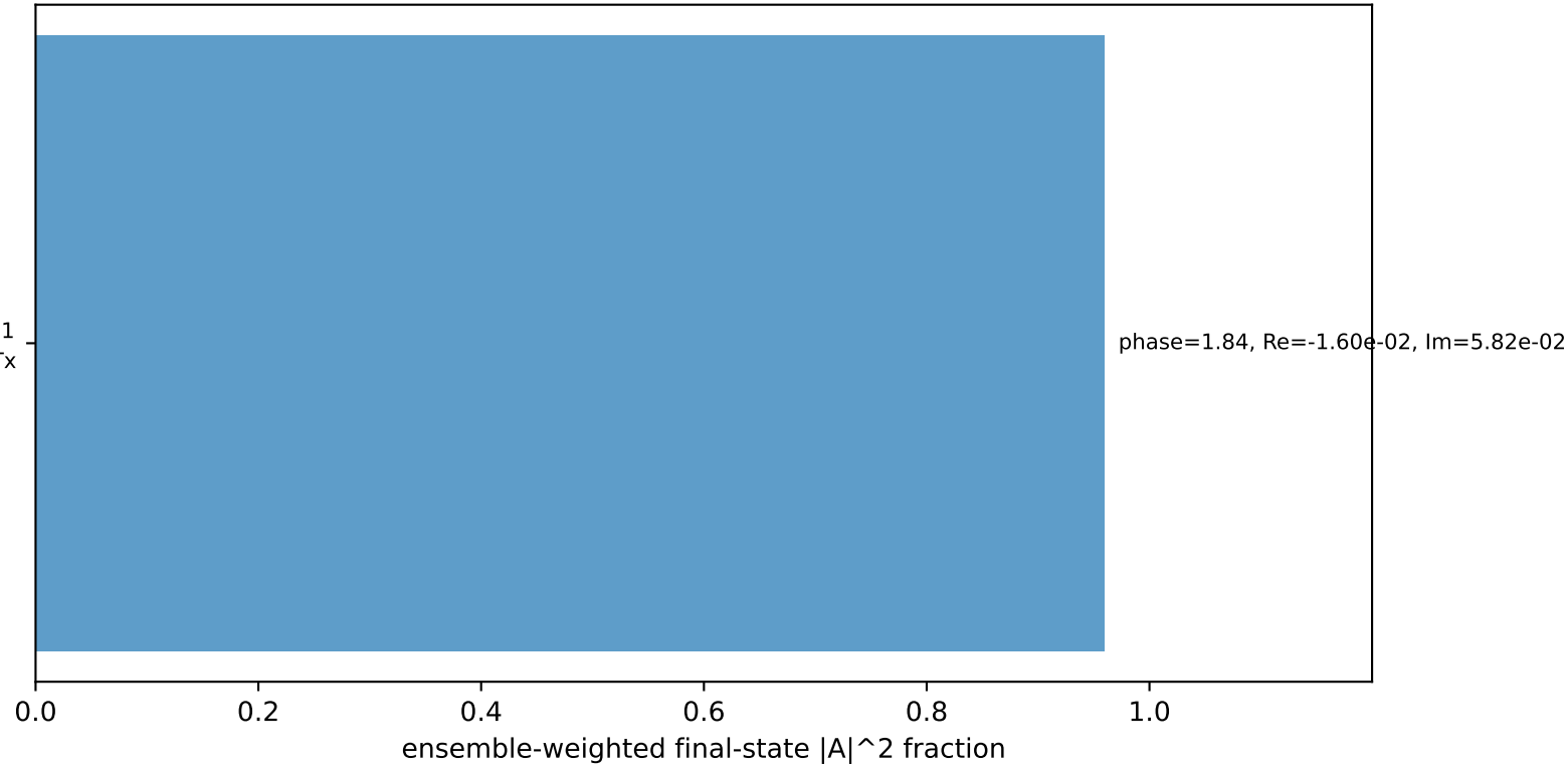
Leading initial-ensemble/final-state components (N=1, retained=96.0%)
