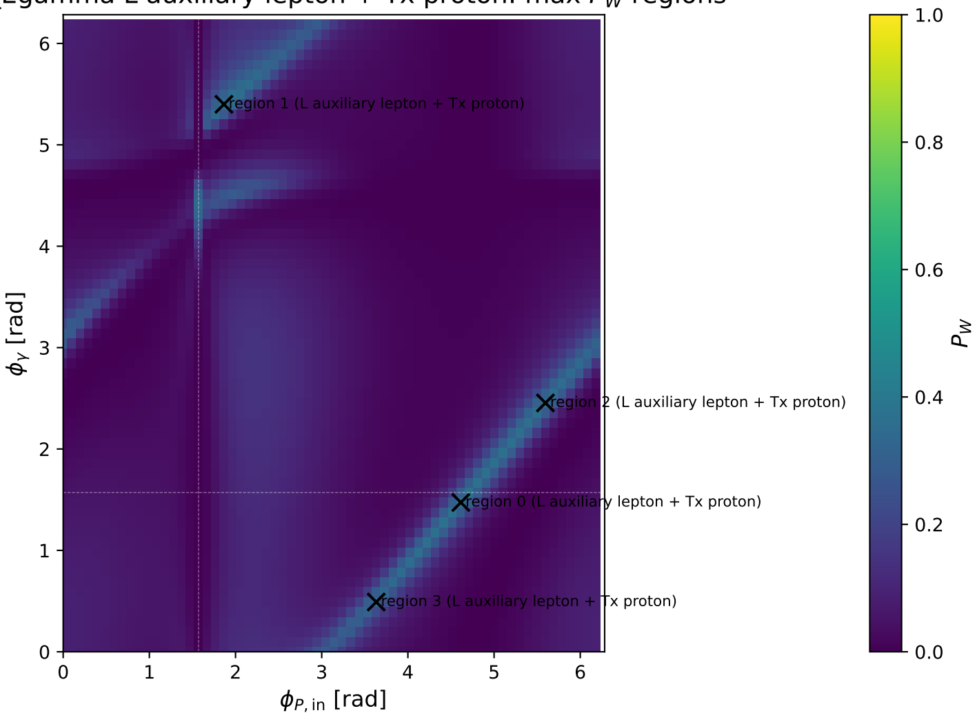
Gamma L auxiliary lepton + Tx proton: max P_W regions
