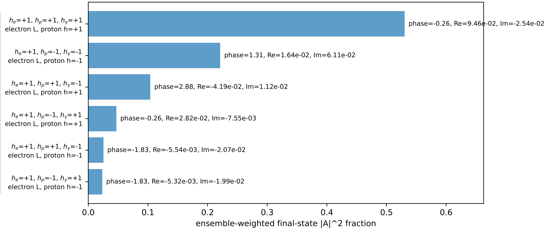
Leading initial-ensemble/final-state components (N=6, retained=95.1%)
