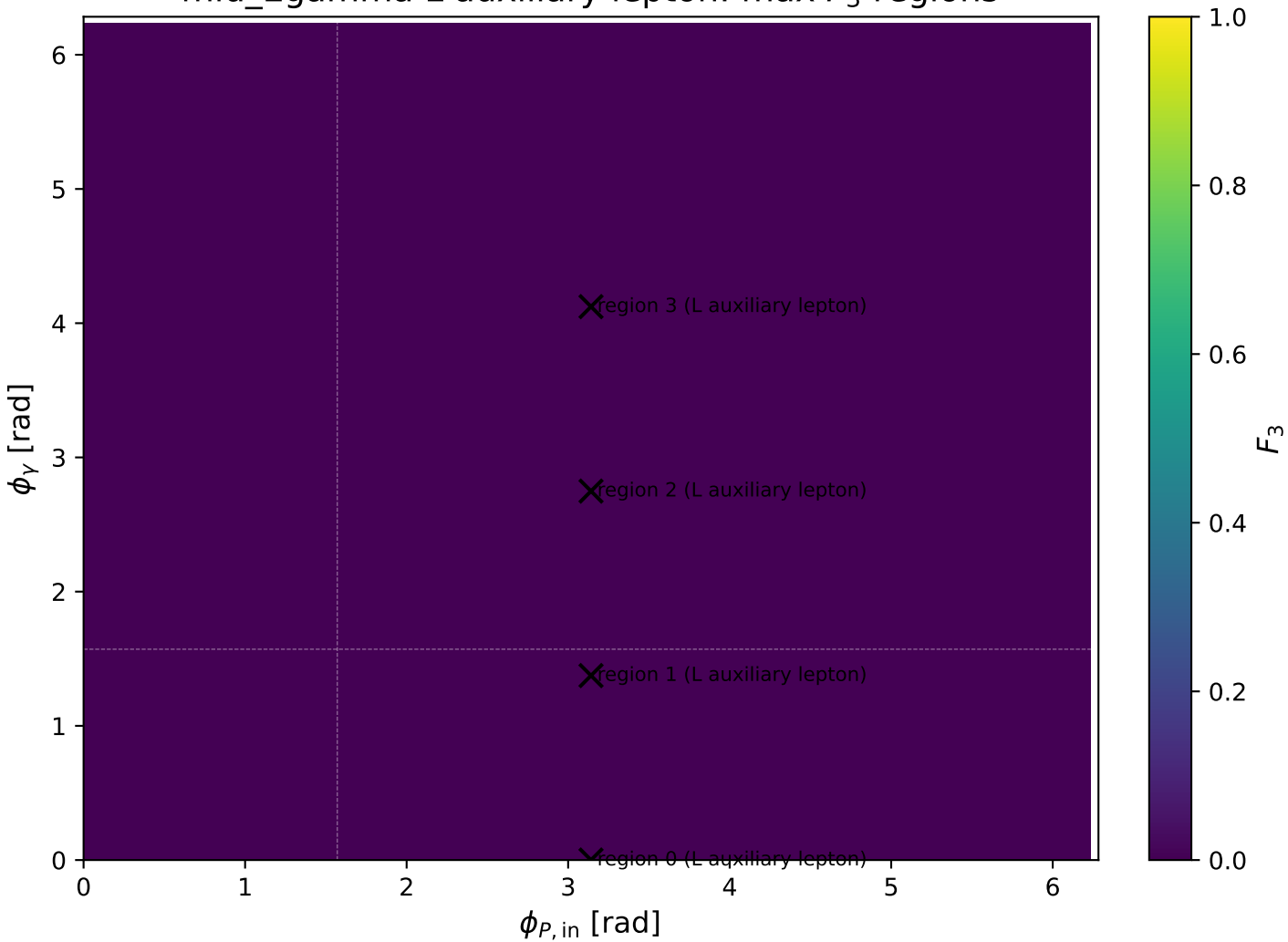
mid_Egamma L auxiliary lepton: max F_3 regions
