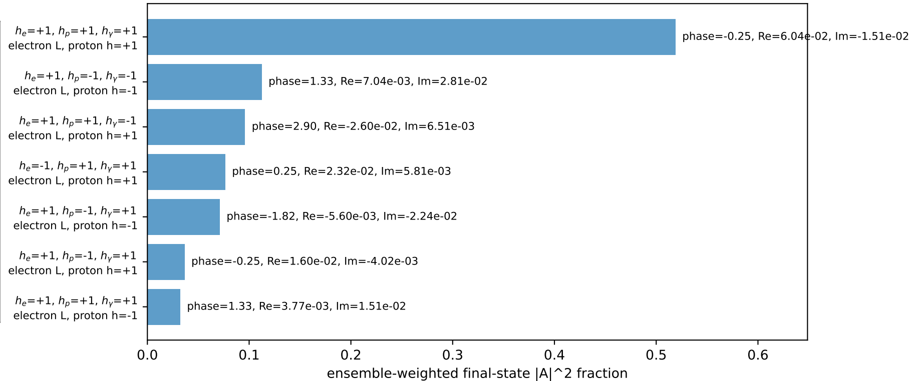
Leading initial-ensemble/final-state components (N=7, retained=94.4%)
