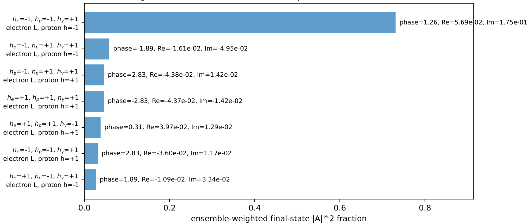
Leading initial-ensemble/final-state components (N=7, retained=97.5%)
