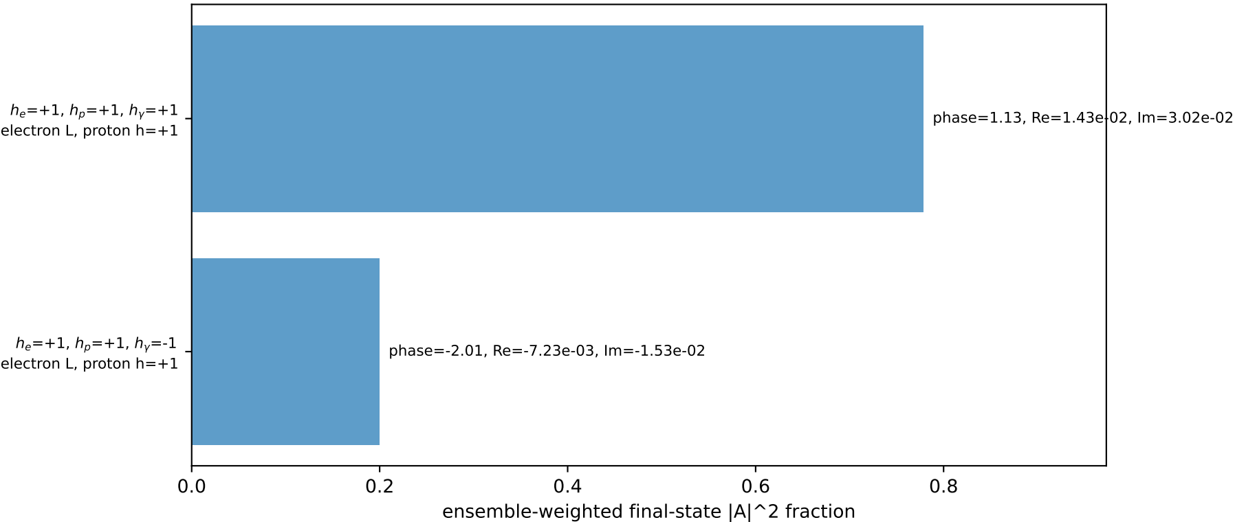
Leading initial-ensemble/final-state components (N=2, retained=97.8%)
