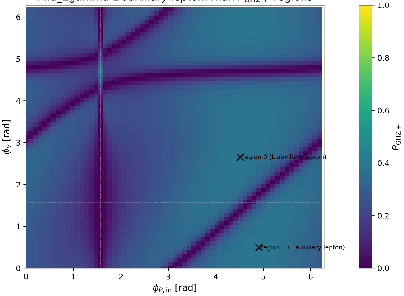
mid_Egamma L auxiliary lepton: max P_{\text{GHZ}+} regions
