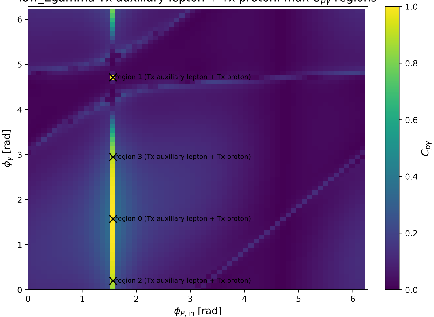
low_Egamma Tx auxiliary lepton + Tx proton: max C_{p\gamma} regions
