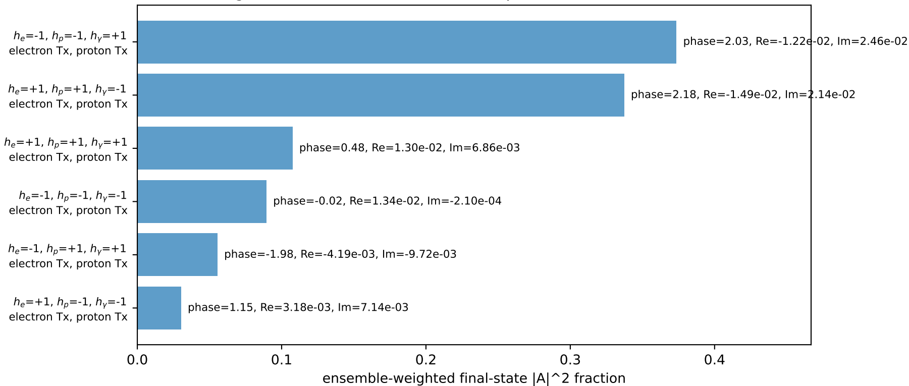
Leading initial-ensemble/final-state components (N=6, retained=99.3%)
