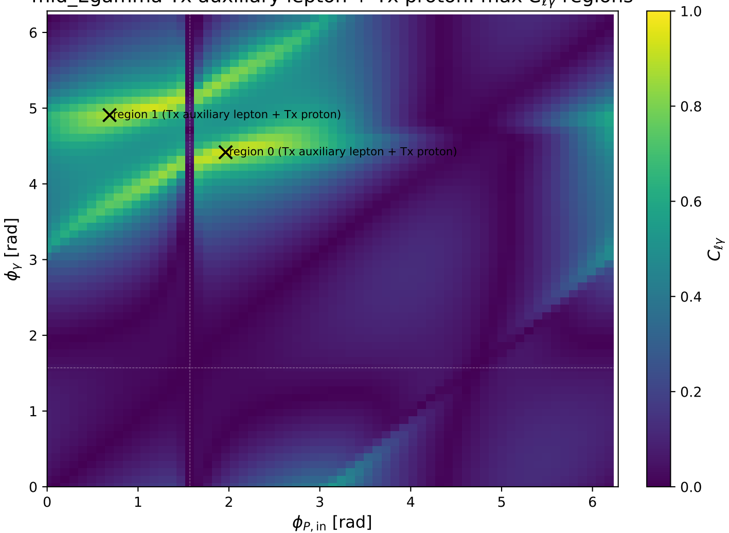
mid_Egamma Tx auxiliary lepton + Tx proton: max C_{\ell\gamma} regions
