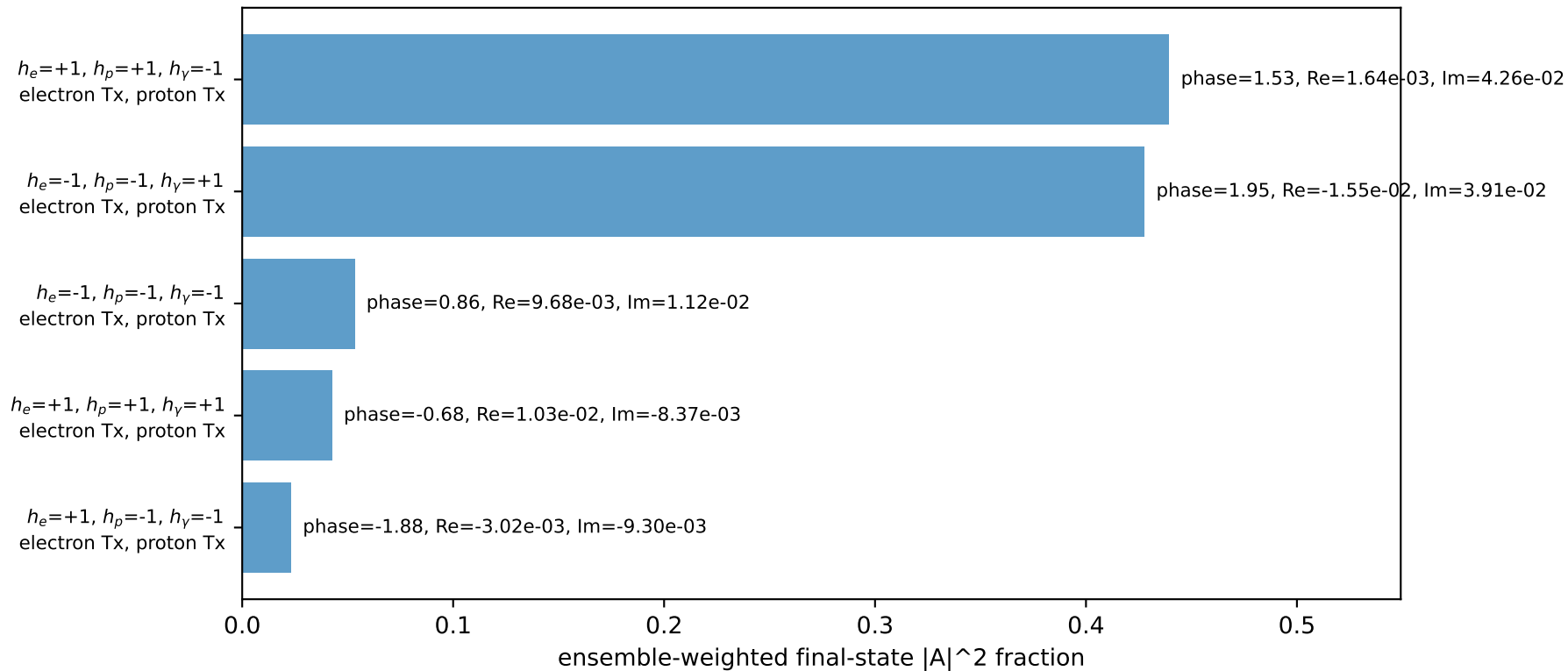
Leading initial-ensemble/final-state components (N=5, retained=98.6%)
