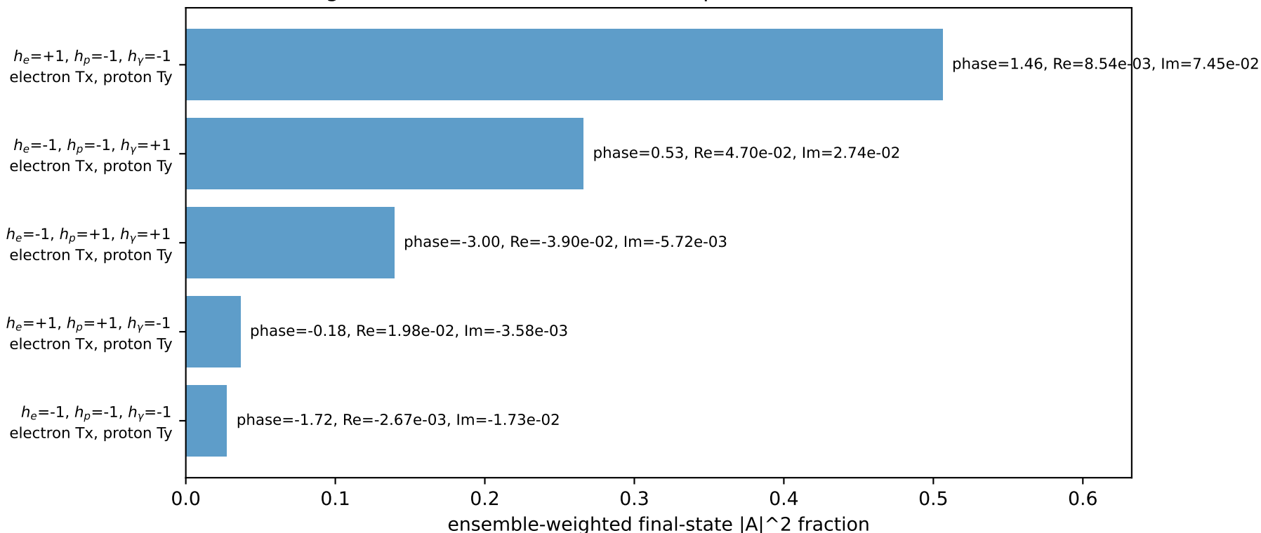
Leading initial-ensemble/final-state components (N=5, retained=97.6%)
