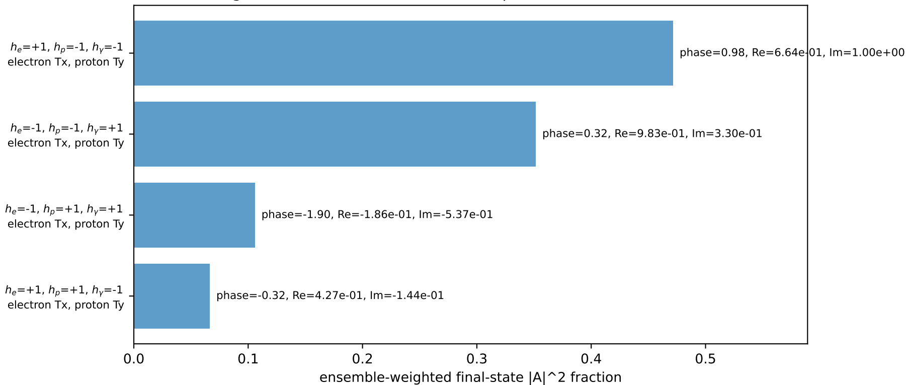
Leading initial-ensemble/final-state components (N=4, retained=99.4%)
