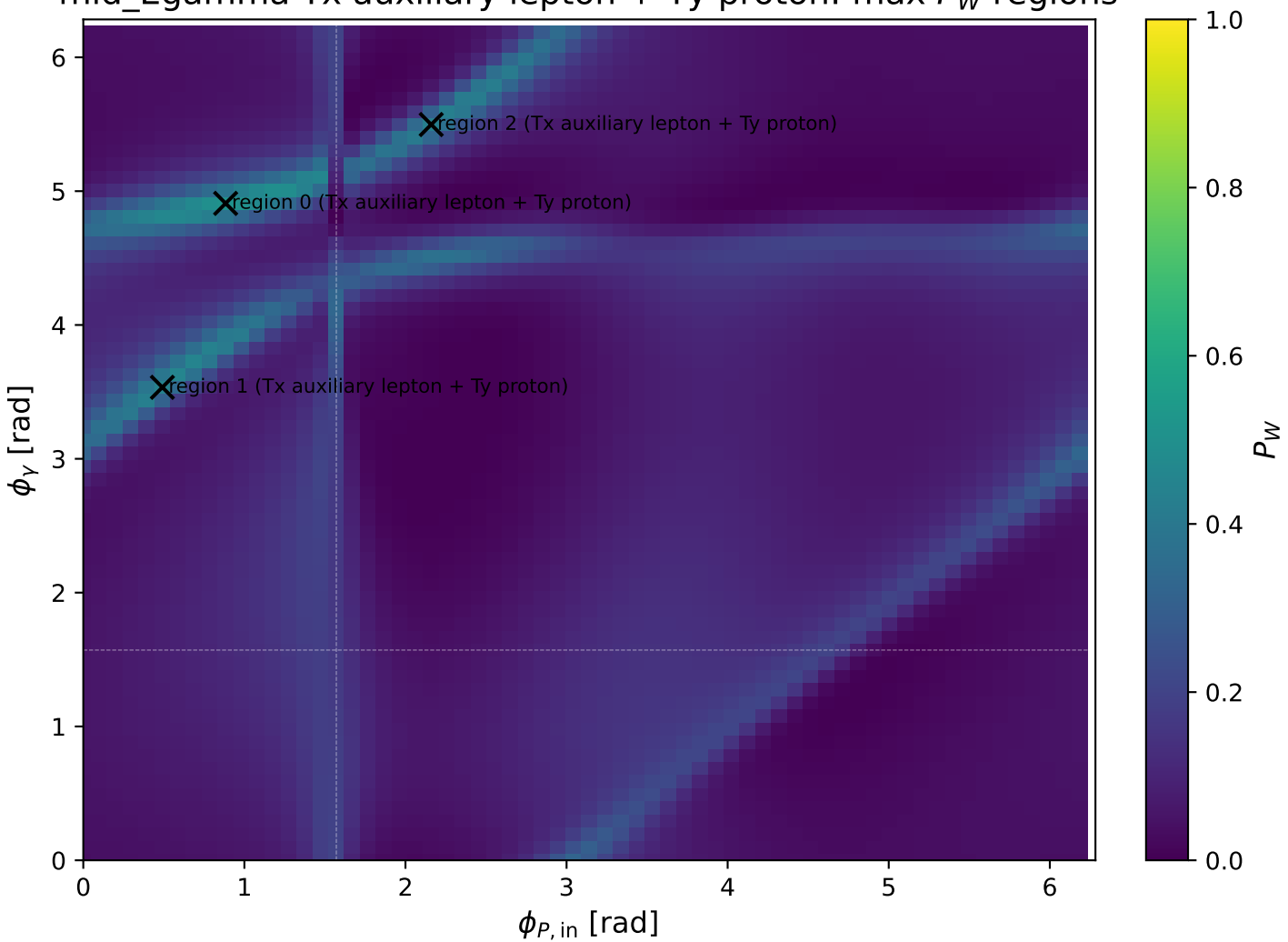
mid_Egamma Tx auxiliary lepton + Ty proton: max P_W regions
