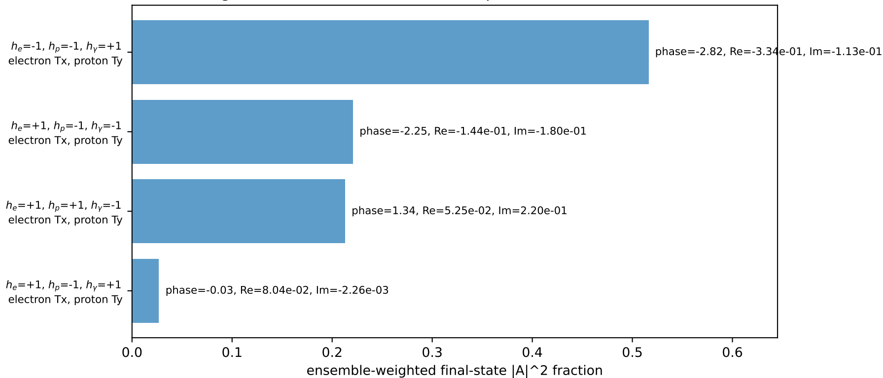
Leading initial-ensemble/final-state components (N=4, retained=97.6%)
