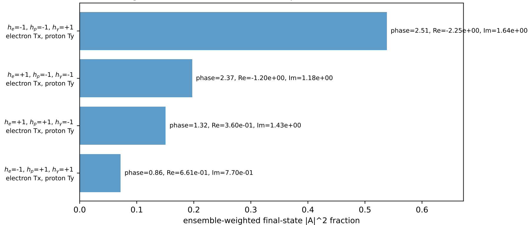
Leading initial-ensemble/final-state components (N=4, retained=95.7%)
