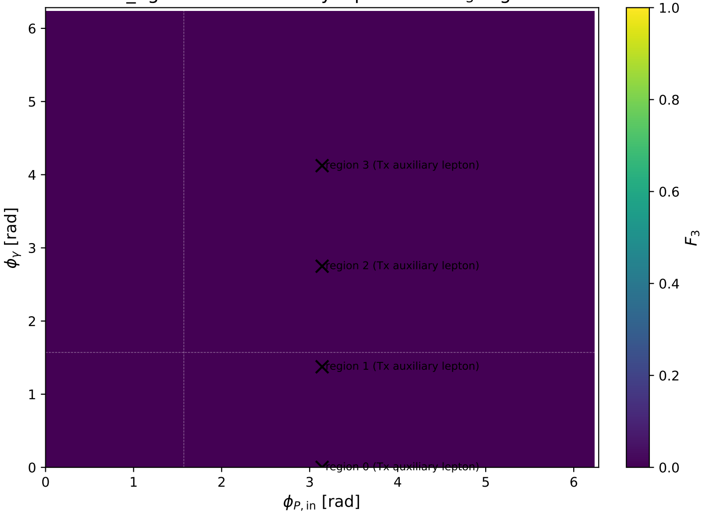
low_Egamma Tx auxiliary lepton: max F_3 regions
