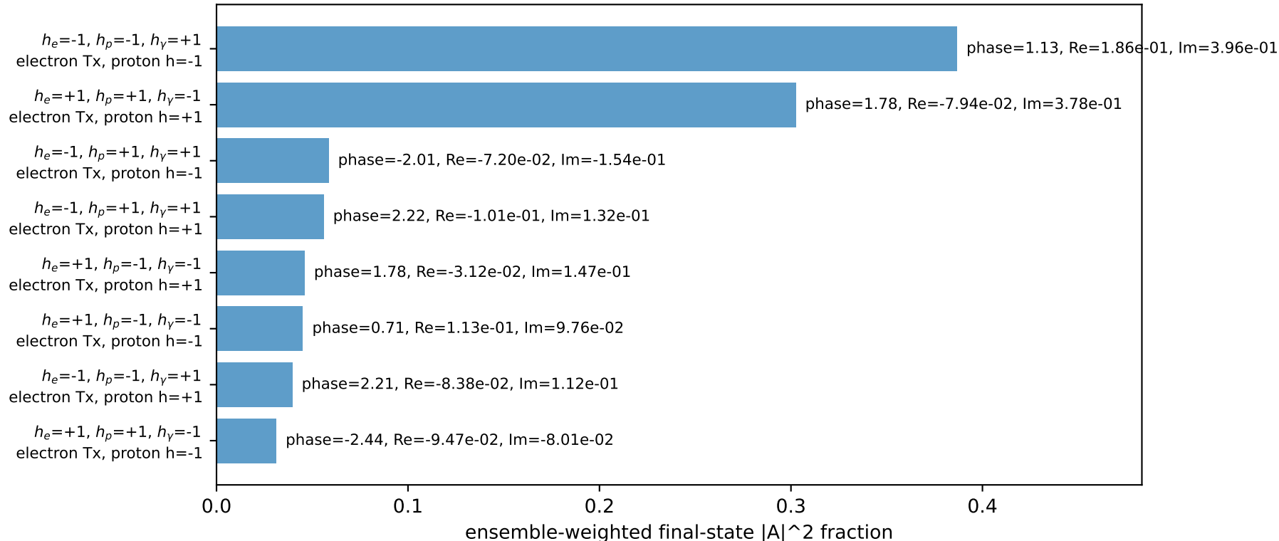
Leading initial-ensemble/final-state components (N=8, retained=96.5%)
