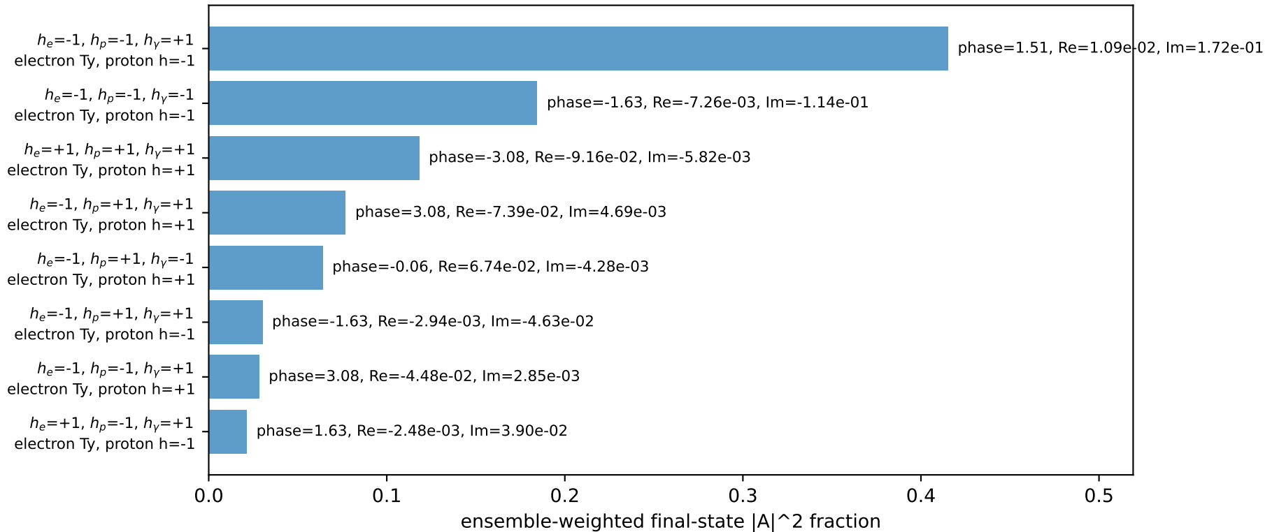
Leading initial-ensemble/final-state components (N=8, retained=93.9%)
