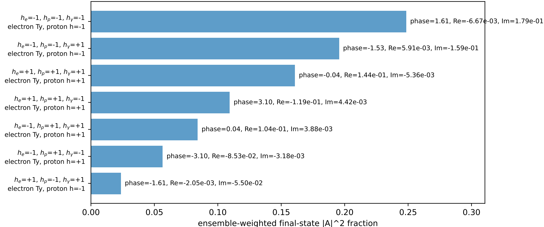
Leading initial-ensemble/final-state components (N=7, retained=87.8%)
