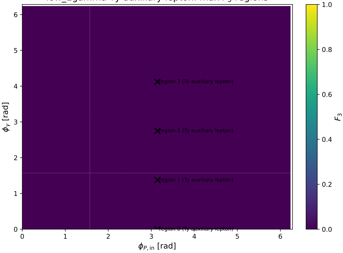
low_Egamma Ty auxiliary lepton: max F_3 regions
