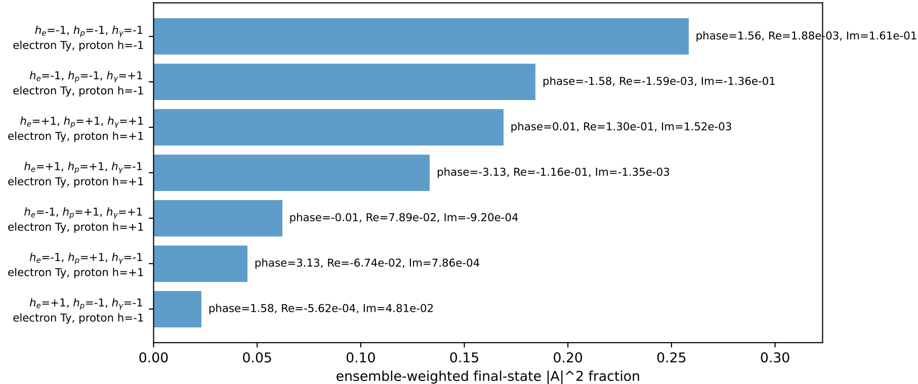
Leading initial-ensemble/final-state components (N=7, retained=87.6%)
