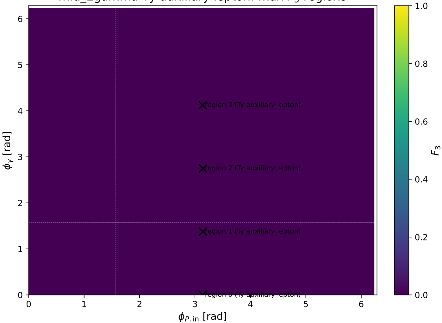
mid_Egamma Ty auxiliary lepton: max F_3 regions
