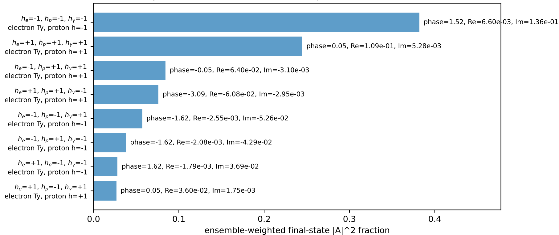
Leading initial-ensemble/final-state components (N=8, retained=93.7%)
