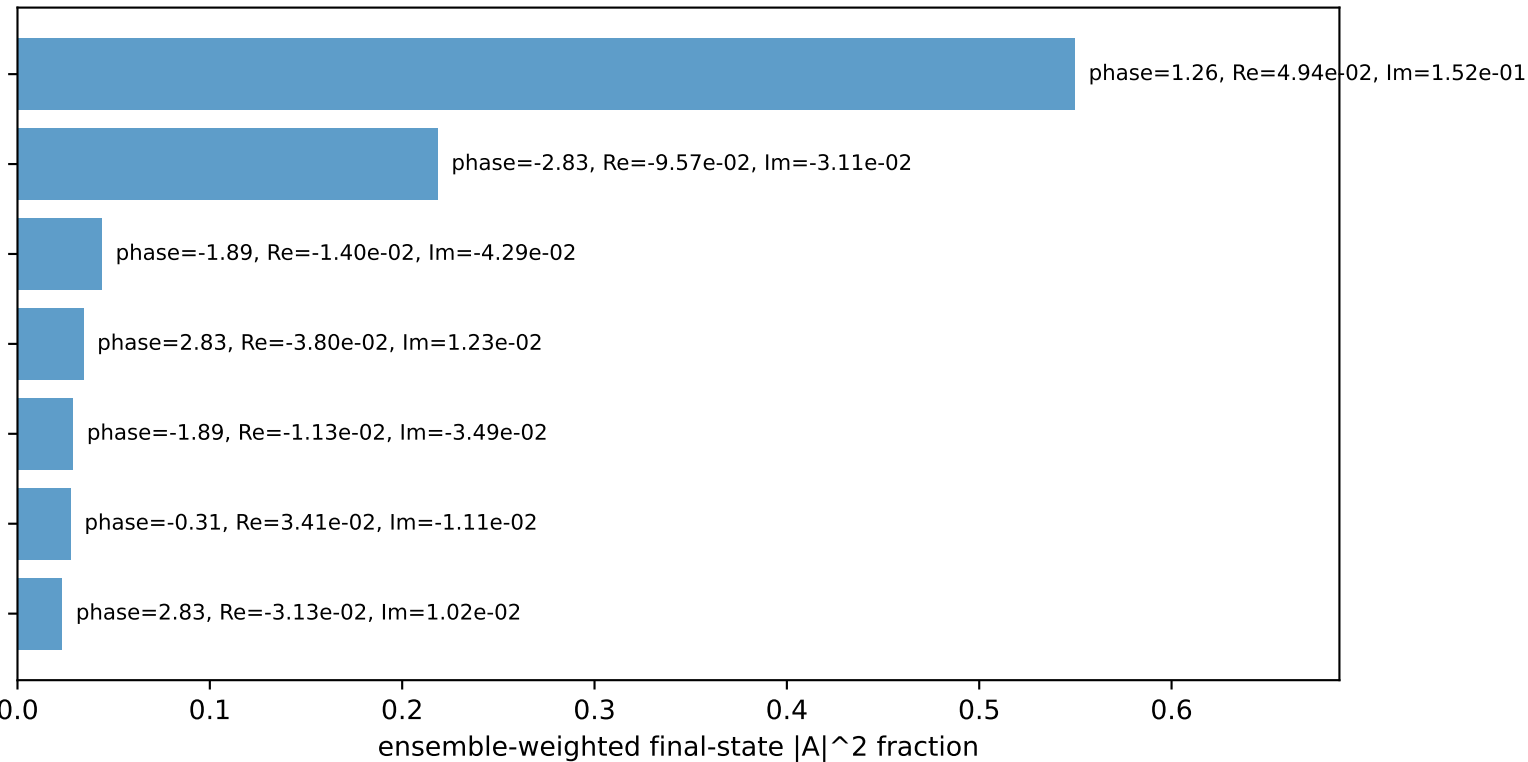
Leading initial-ensemble/final-state components (N=7, retained=92.7%)
