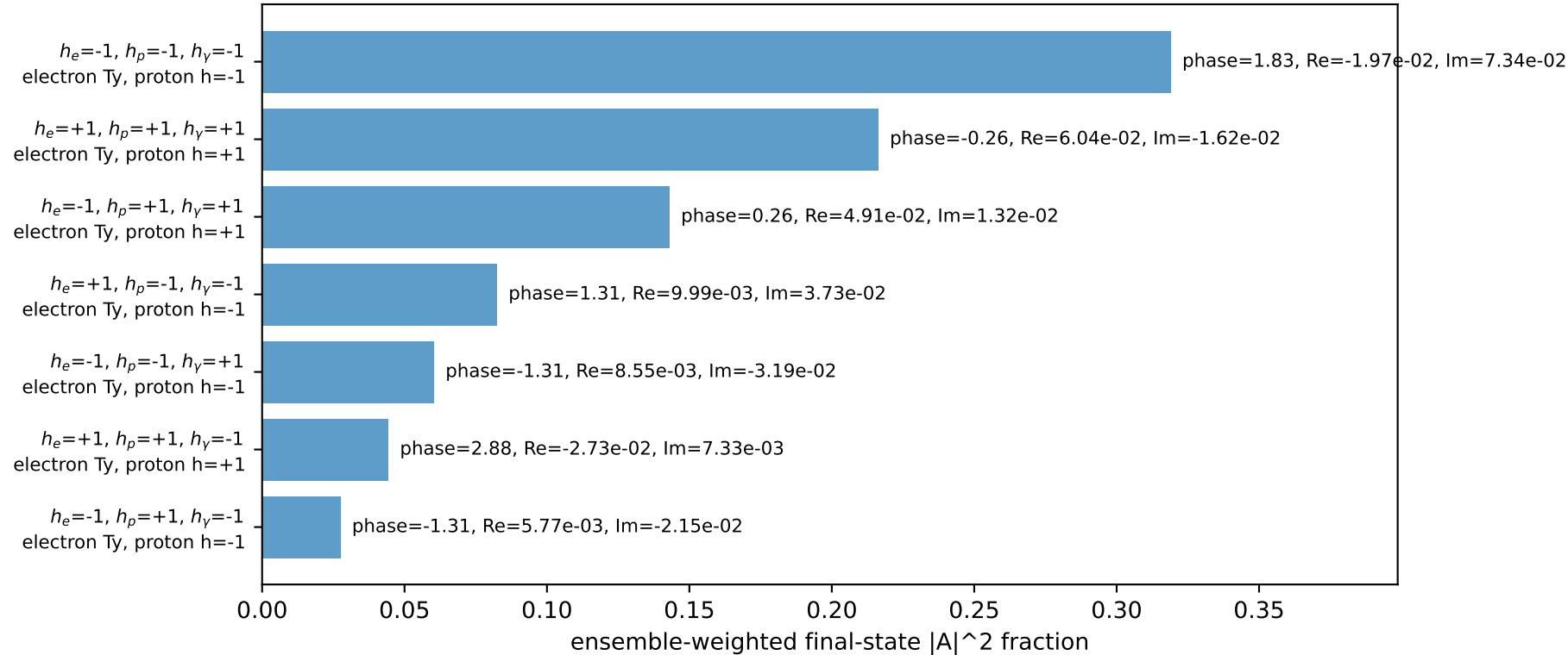
Leading initial-ensemble/final-state components (N=7, retained=89.3%)
