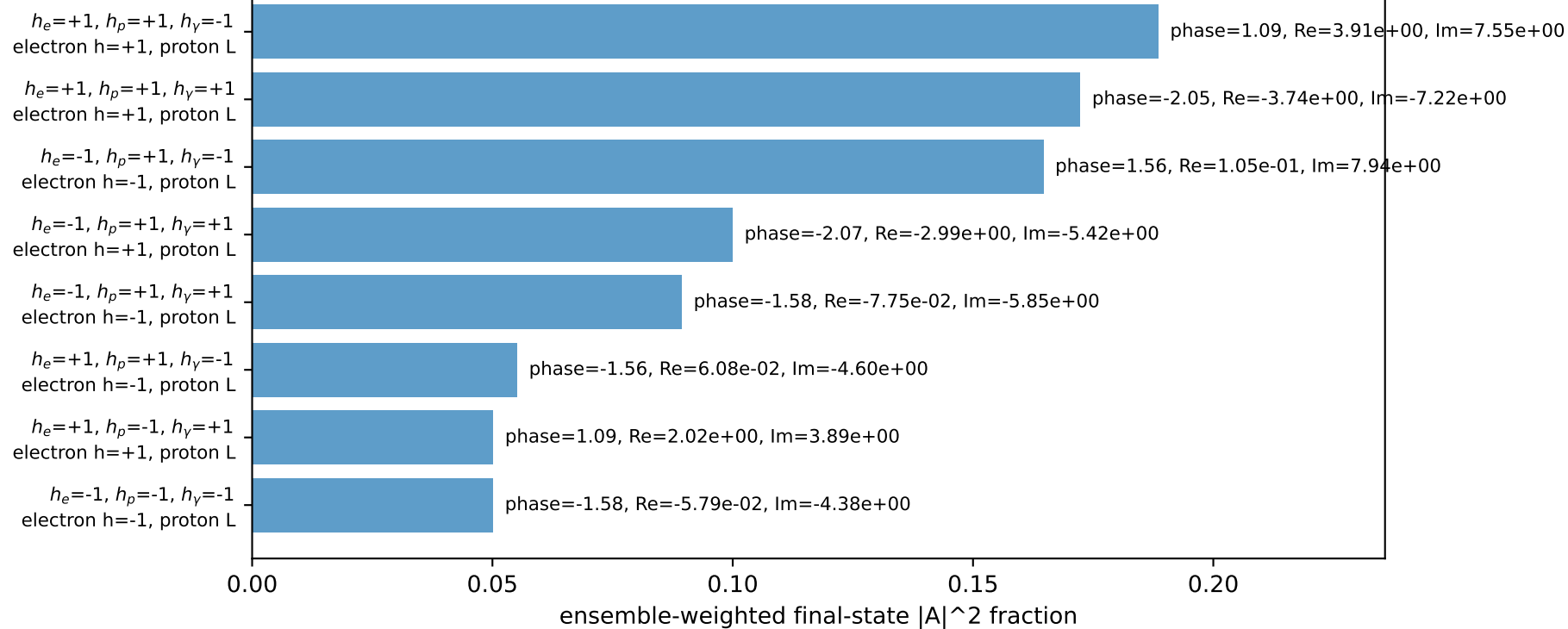
Leading initial-ensemble/final-state components (N=8, retained=87.1%)
