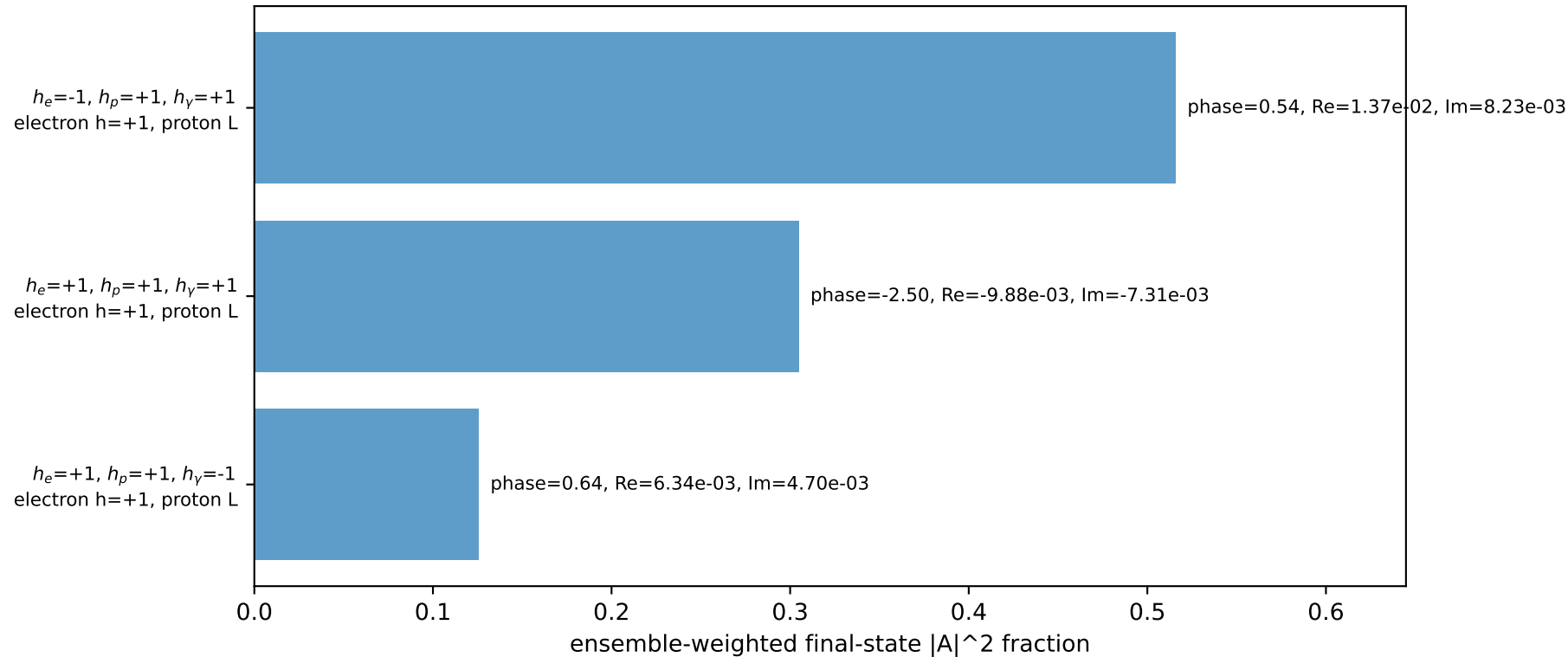
Leading initial-ensemble/final-state components (N=3, retained=94.6%)
