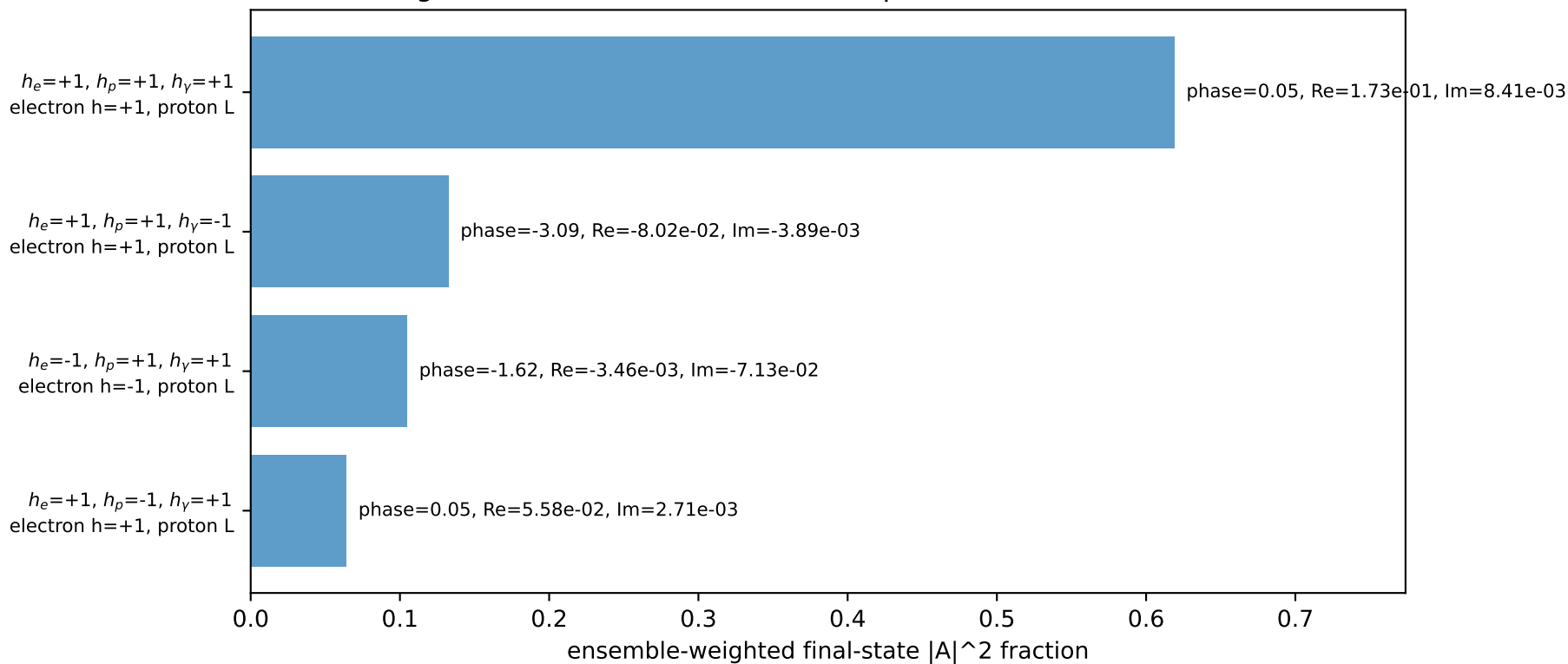
Leading initial-ensemble/final-state components (N=4, retained=92.1%)
