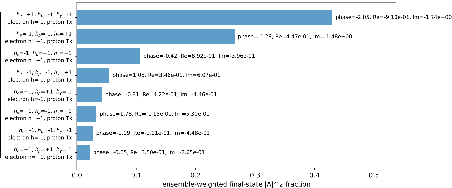
Leading initial-ensemble/final-state components (N=8, retained=97.9%)
