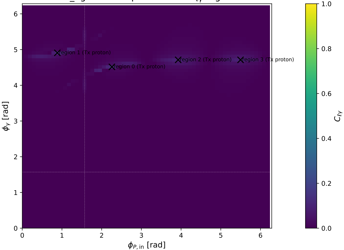
low_Egamma Tx proton: max C_{\ell\gamma} regions
