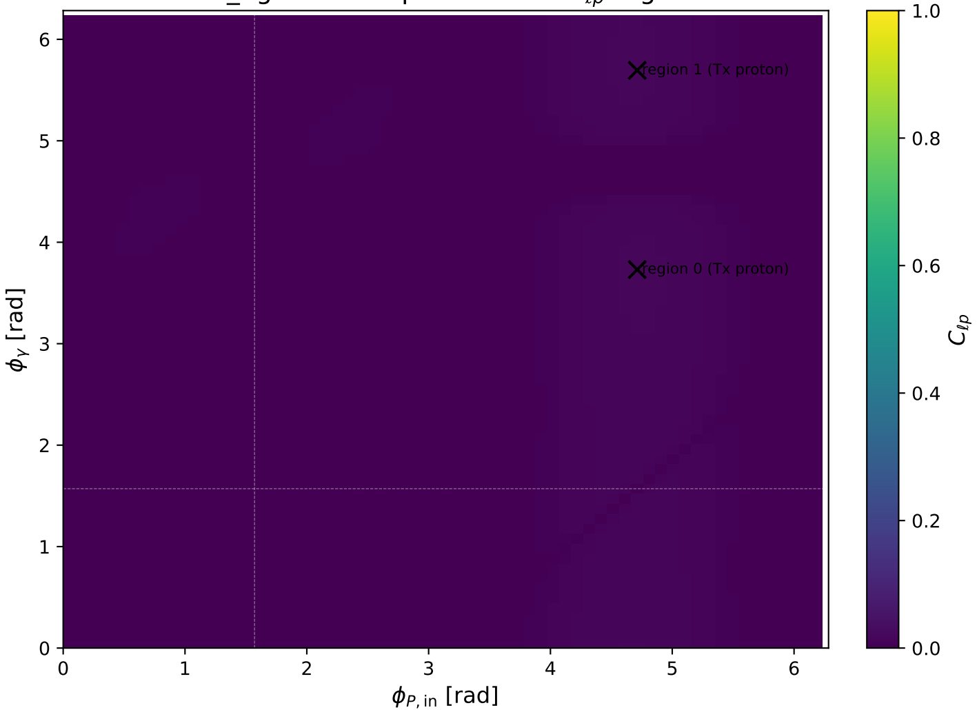
low_Egamma Tx proton: max C_{lp} regions
