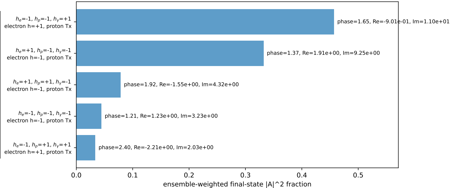
Leading initial-ensemble/final-state components (N=5, retained=94.6%)
