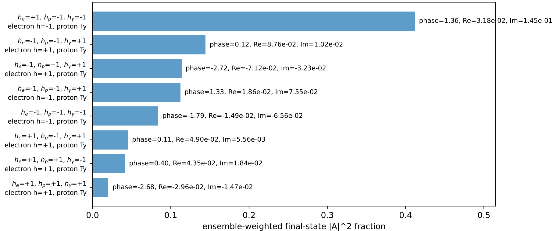
Leading initial-ensemble/final-state components (N=8, retained=97.3%)
