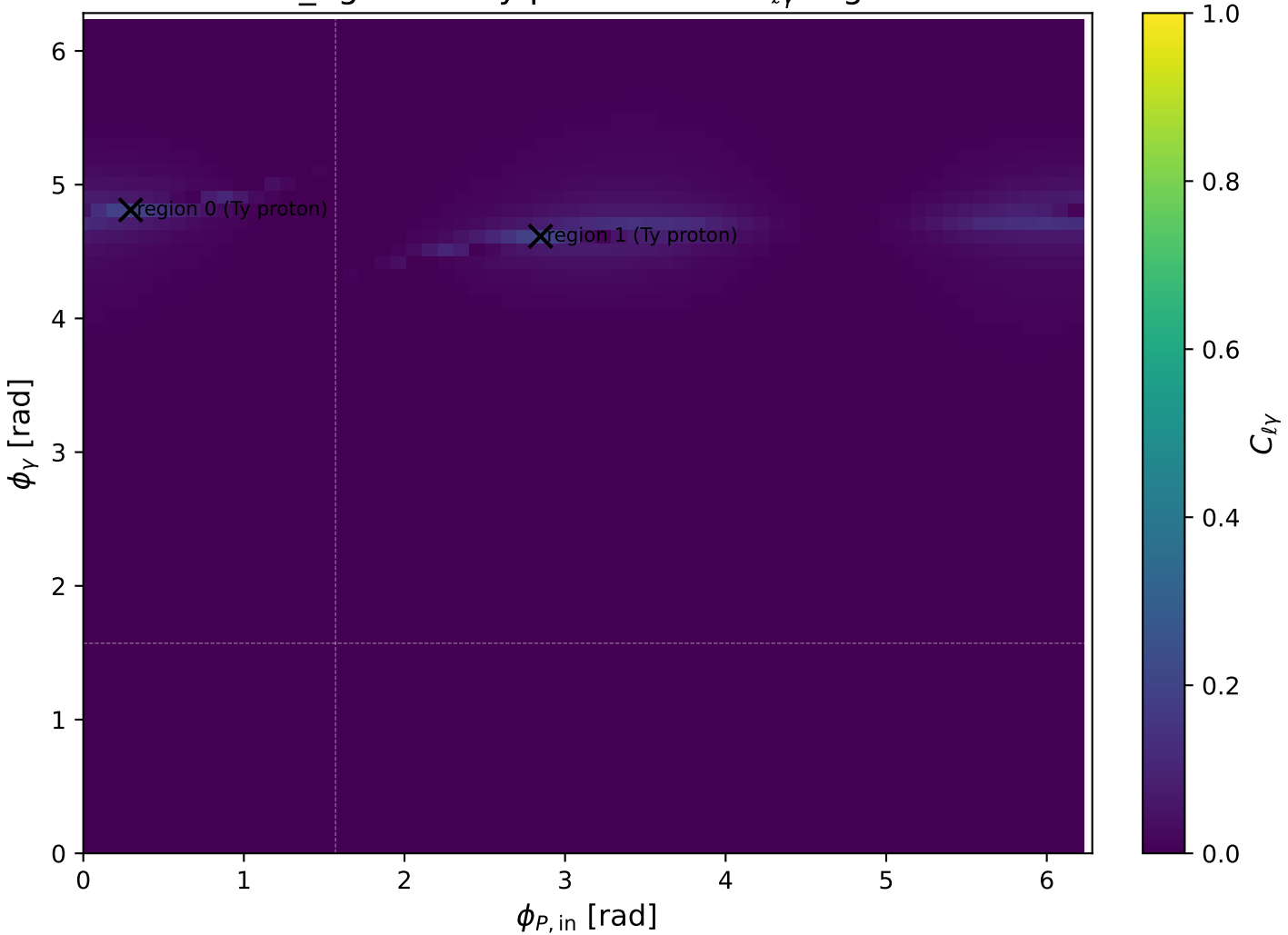
low_Egamma Ty proton: max C_{\ell\gamma} regions
