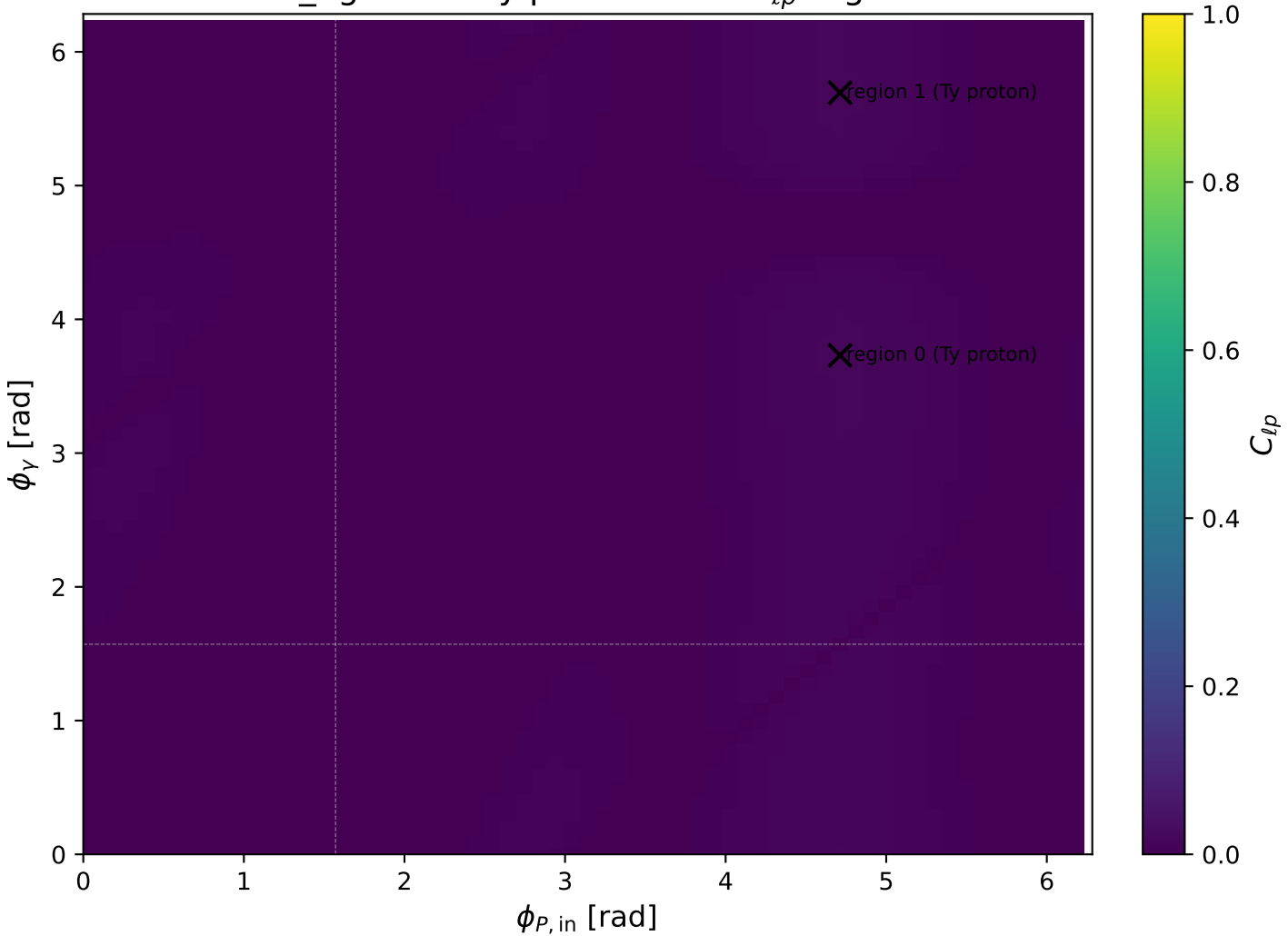
low_Egamma Ty proton: max C_{lp} regions
