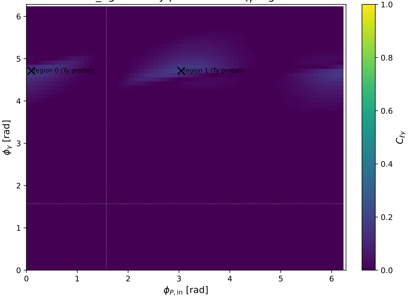
mid_Egamma Ty proton: max C_{\ell\gamma} regions
