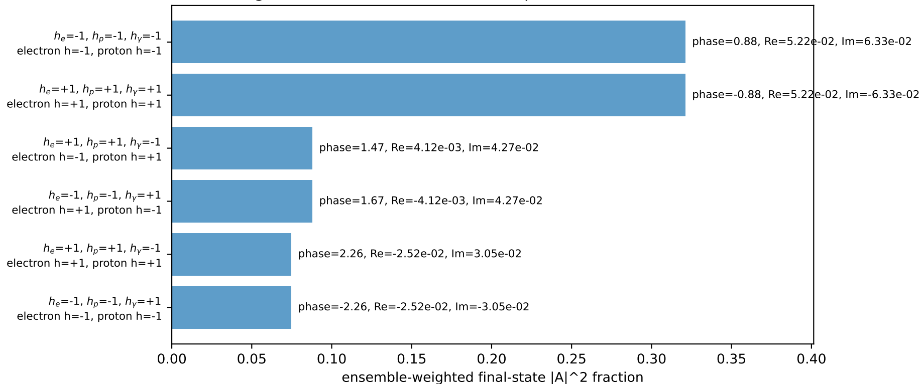
Leading initial-ensemble/final-state components (N=6, retained=96.7%)
