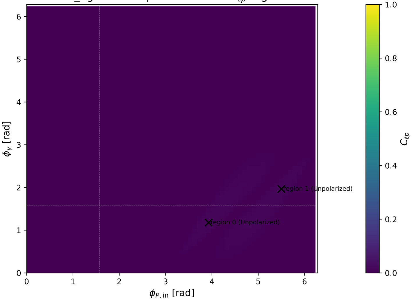
mid_Egamma Unpolarized: max C_{lp} regions
