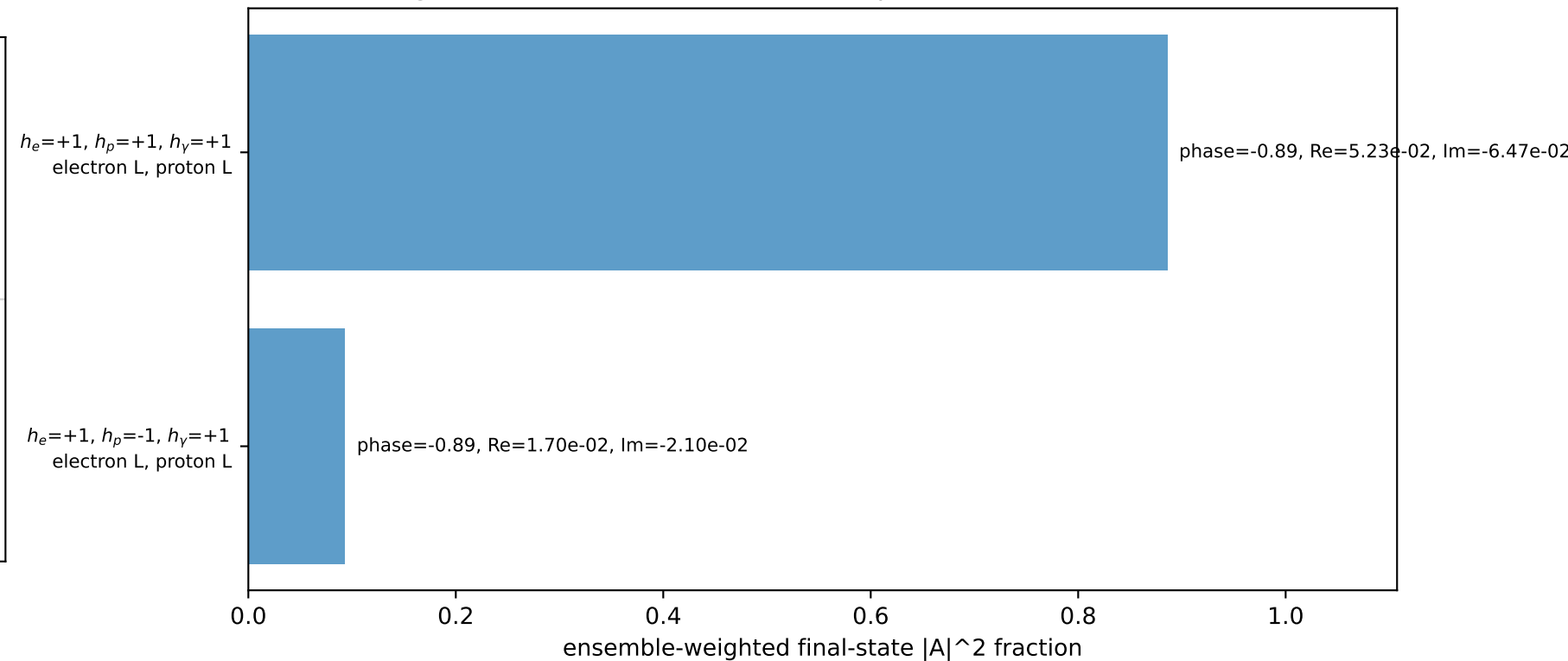
Leading initial-ensemble/final-state components (N=2, retained=97.9%)
