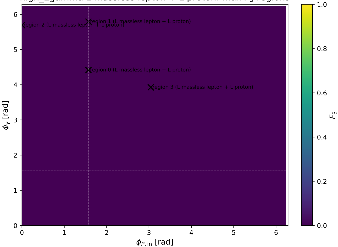
high_Egamma L massless lepton + L proton: max F_3 regions
