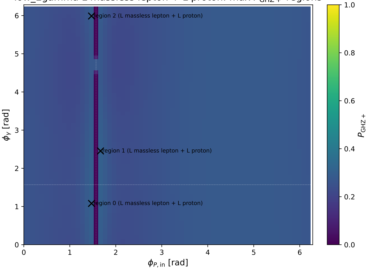
low_Egamma L massless lepton + L proton: max P_{\text{GHZ}+} regions
