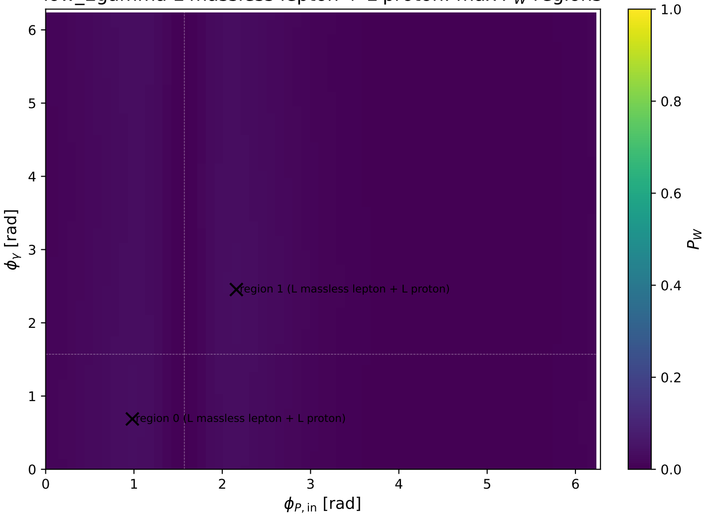
low_Egamma L massless lepton + L proton: max P_W regions
