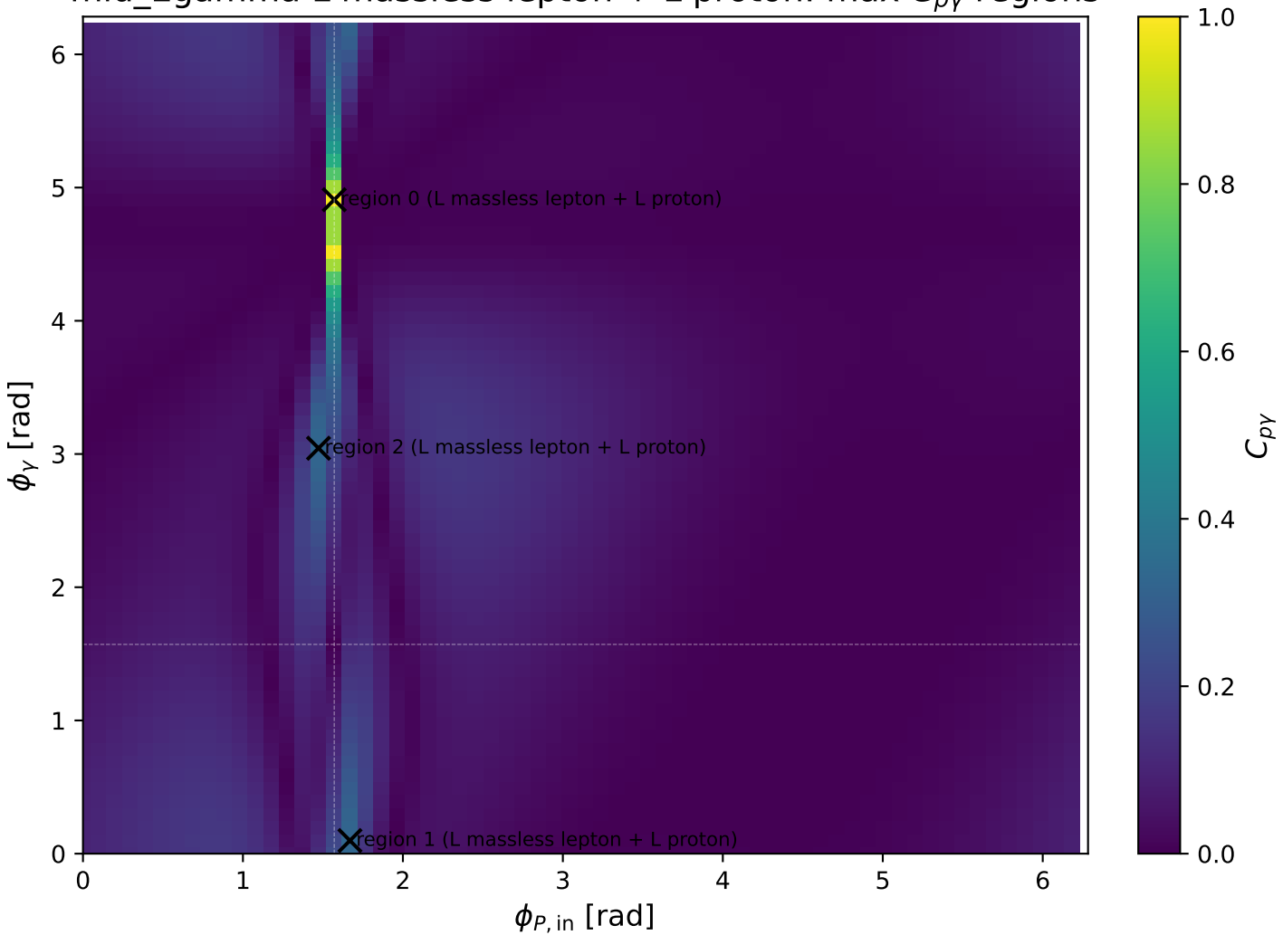
mid_Egamma L massless lepton + L proton: max C_{p\gamma} regions
