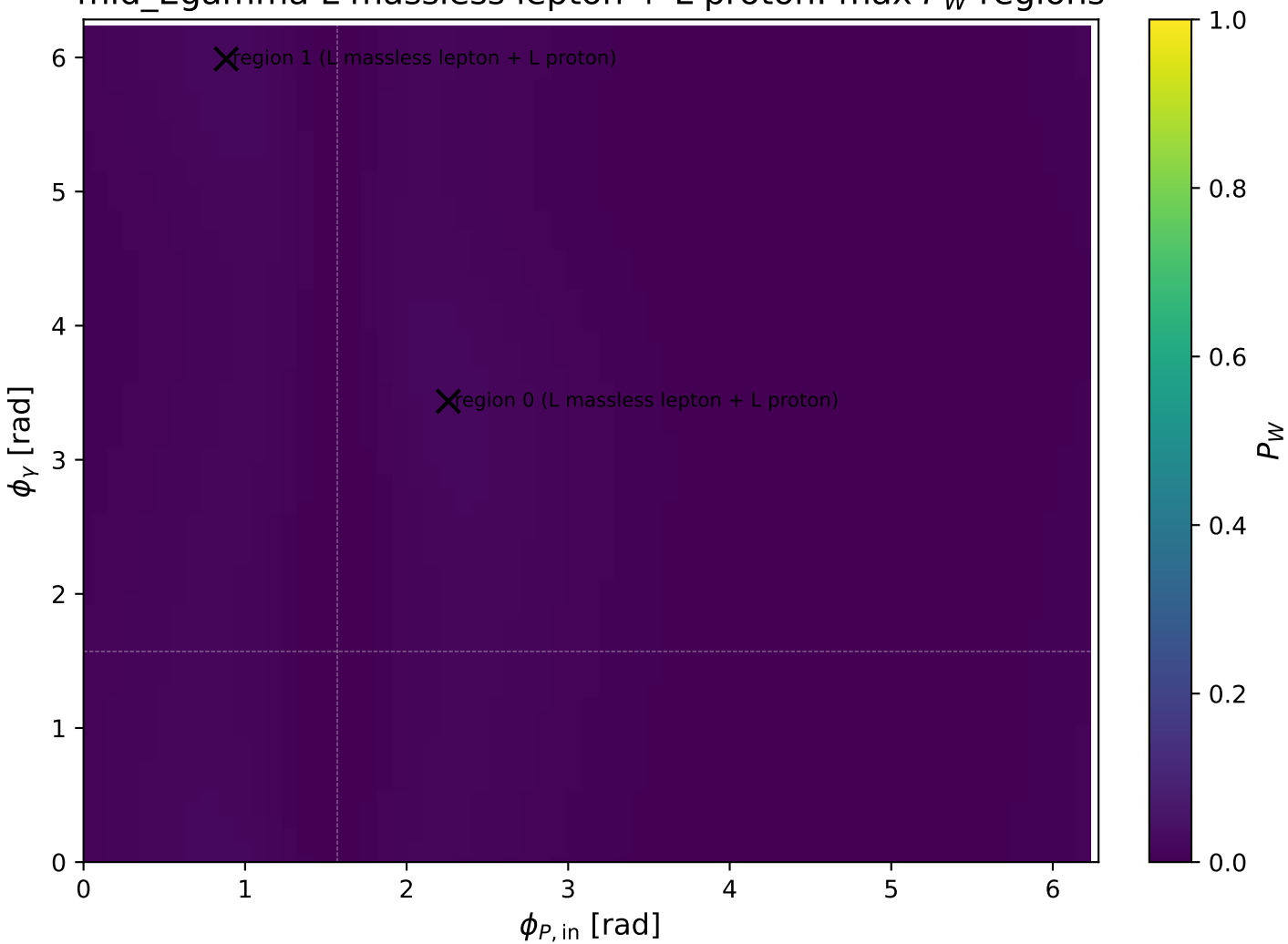
mid_Egamma L massless lepton + L proton: max P_W regions
