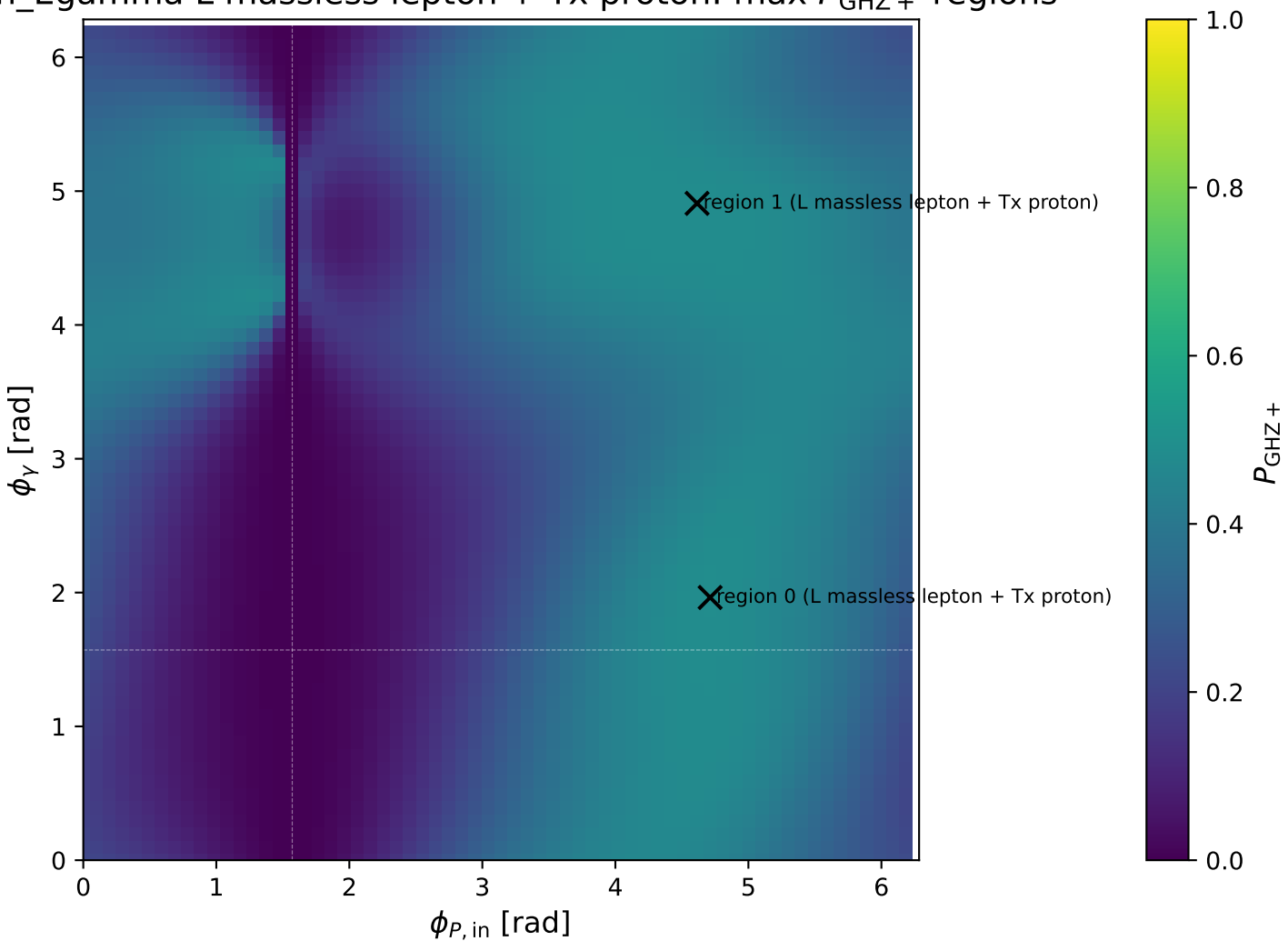
\gamma L massless lepton + Tx proton: max P_{\text{GHZ}} + regions
