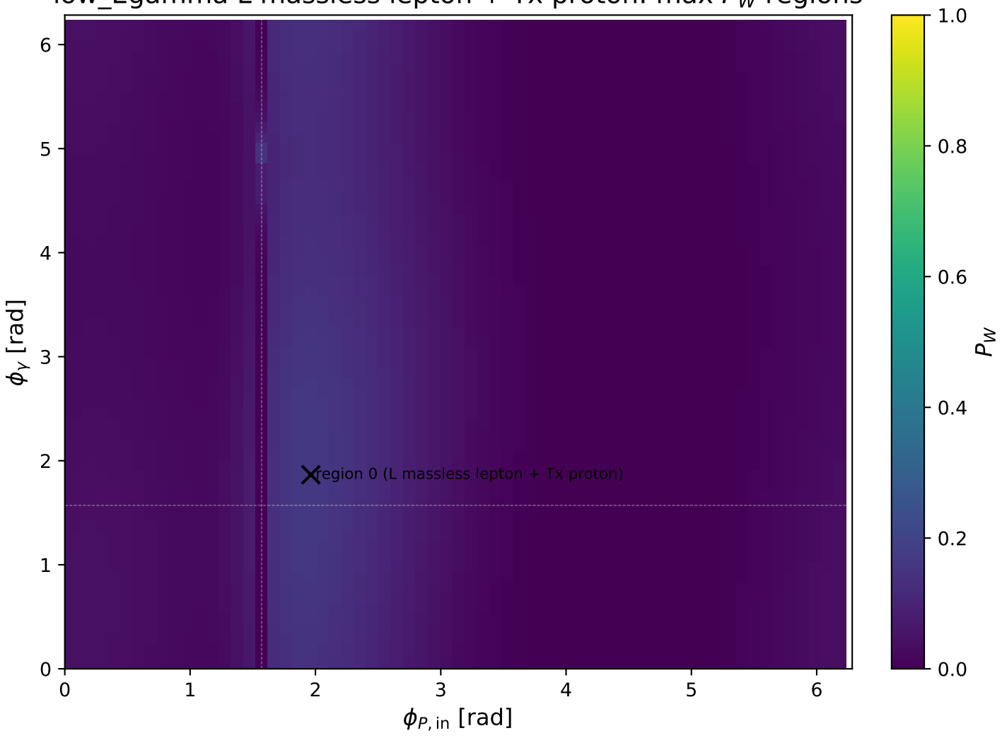
low_Egamma L massless lepton + Tx proton: max P_W regions
