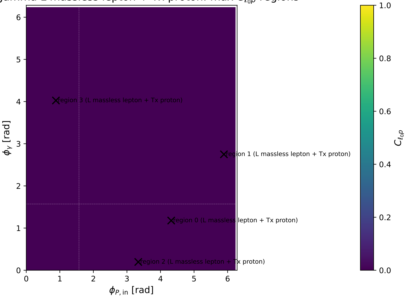
gamma L massless lepton + Tx proton: max C_{\ell_0 p} regions
