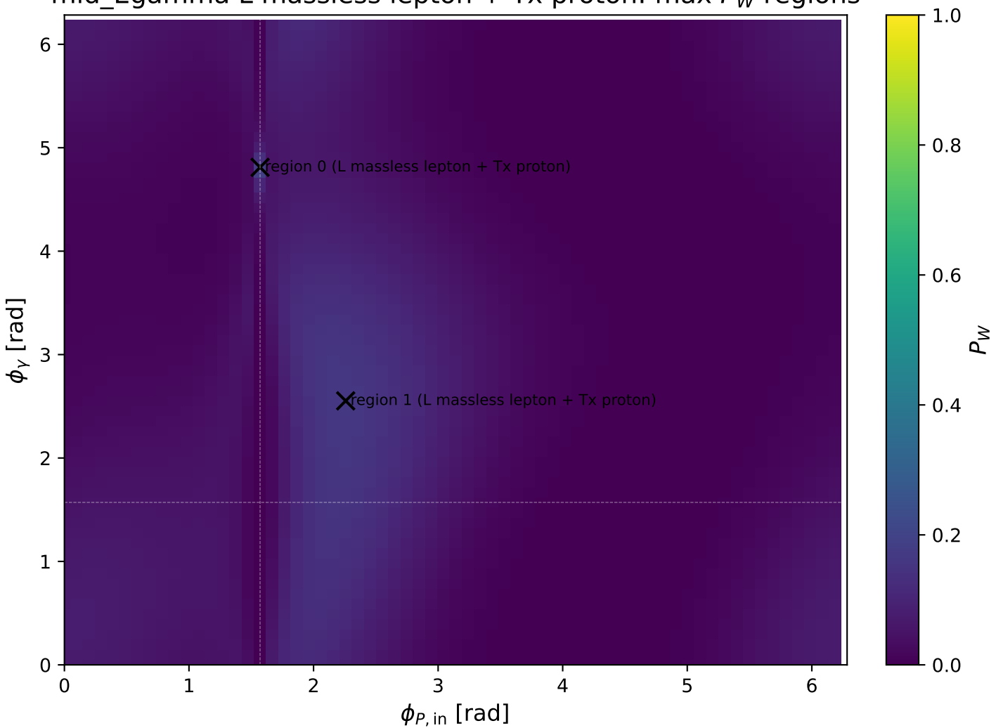
mid_Egamma L massless lepton + Tx proton: max P_W regions
