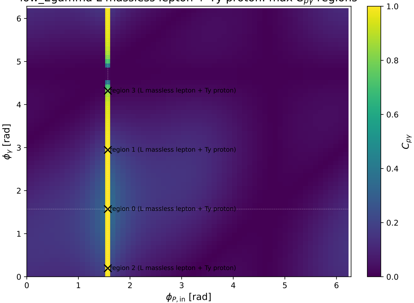
low_Egamma L massless lepton + Ty proton: max C_{p\gamma} regions
