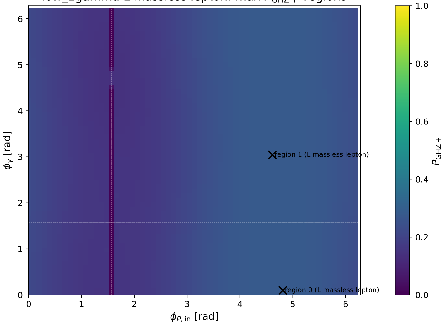
low_Egamma L massless lepton: max P_{\text{GHZ}+} regions
