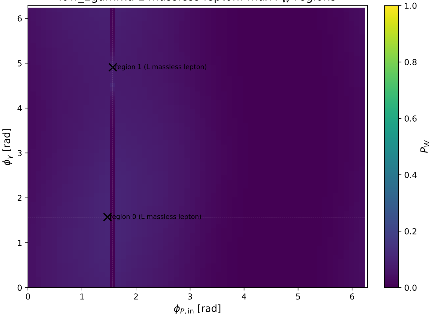
low_Egamma L massless lepton: max P_W regions
