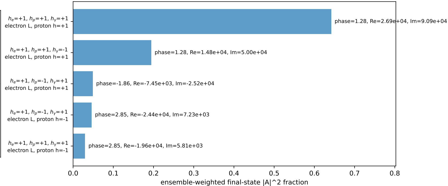
Leading initial-ensemble/final-state components (N=5, retained=96.2%)
