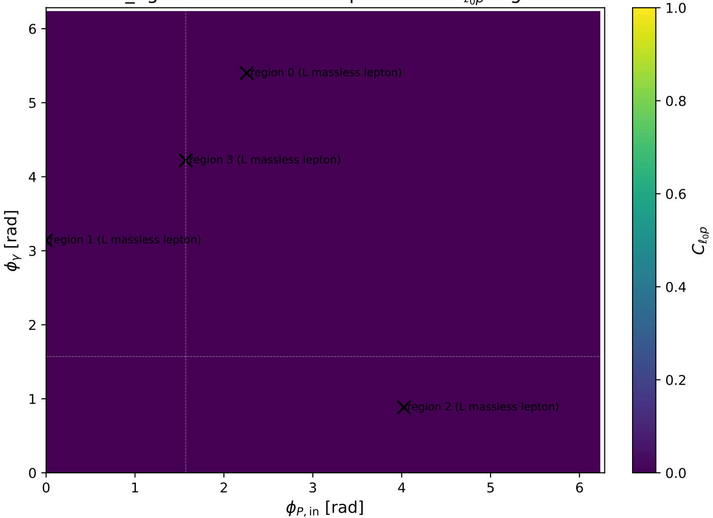
mid_Egamma L massless lepton: max C_{\ell_0 p} regions
