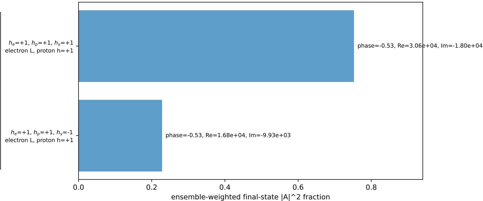
Leading initial-ensemble/final-state components (N=2, retained=98.1%)
