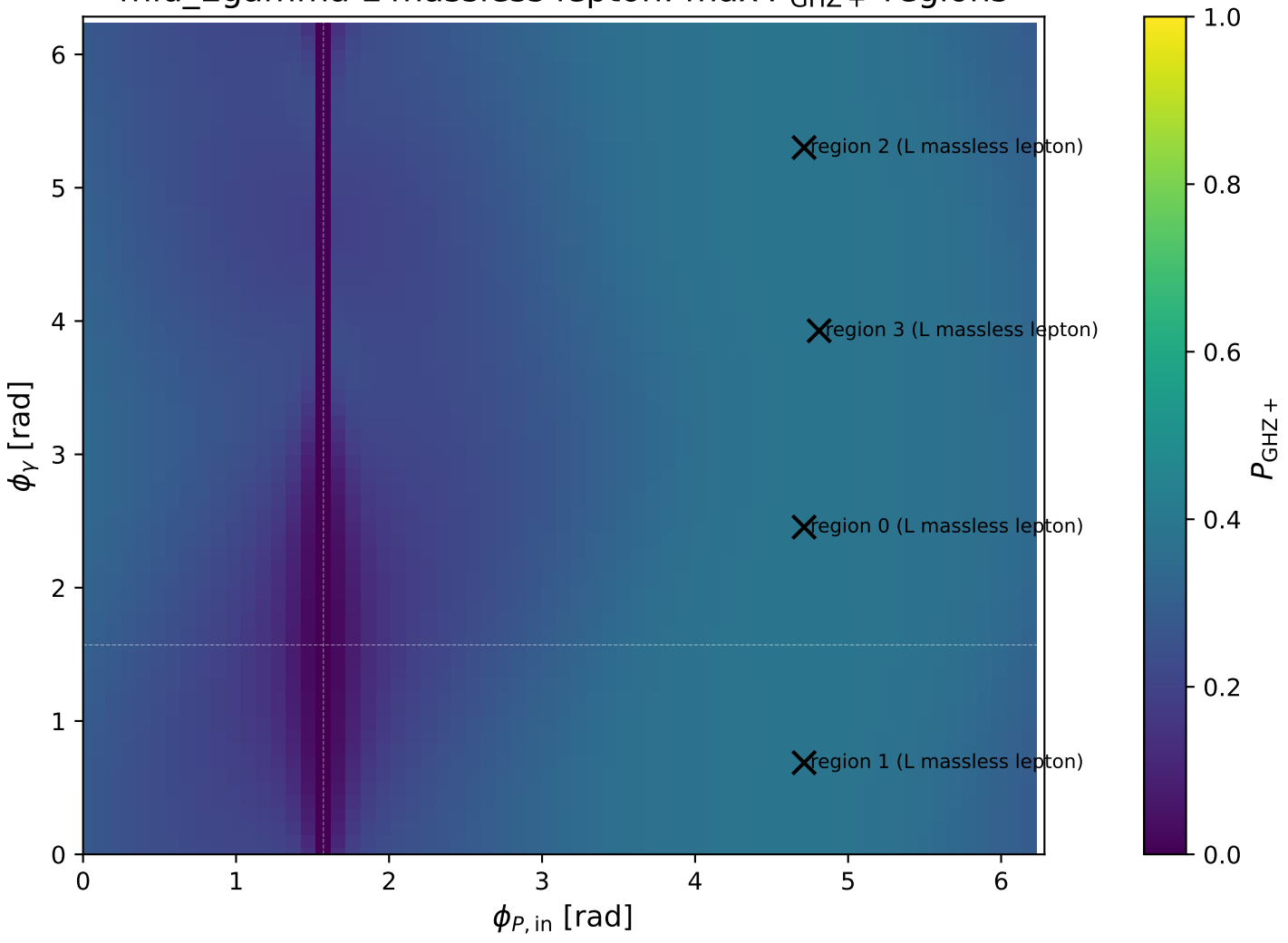
mid_Egamma L massless lepton: max P_{\text{GHZ}+} regions
