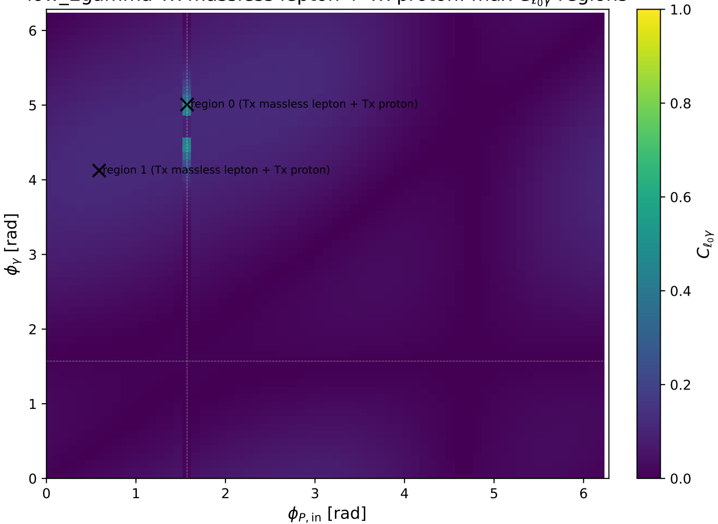
low_Egamma Tx massless lepton + Tx proton: max C_{\ell_0\gamma} regions
