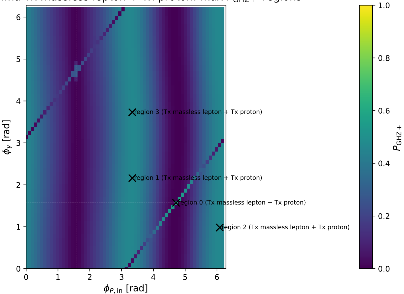
Gamma Tx massless lepton + Tx proton: max P_{\text{GHz}+} regions
