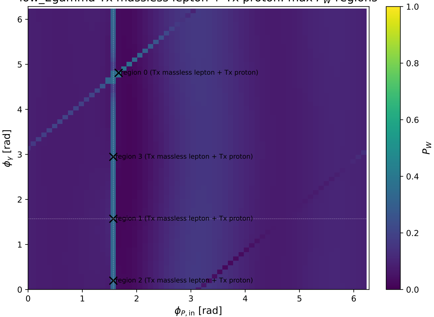
low_Egamma Tx massless lepton + Tx proton: max P_W regions
