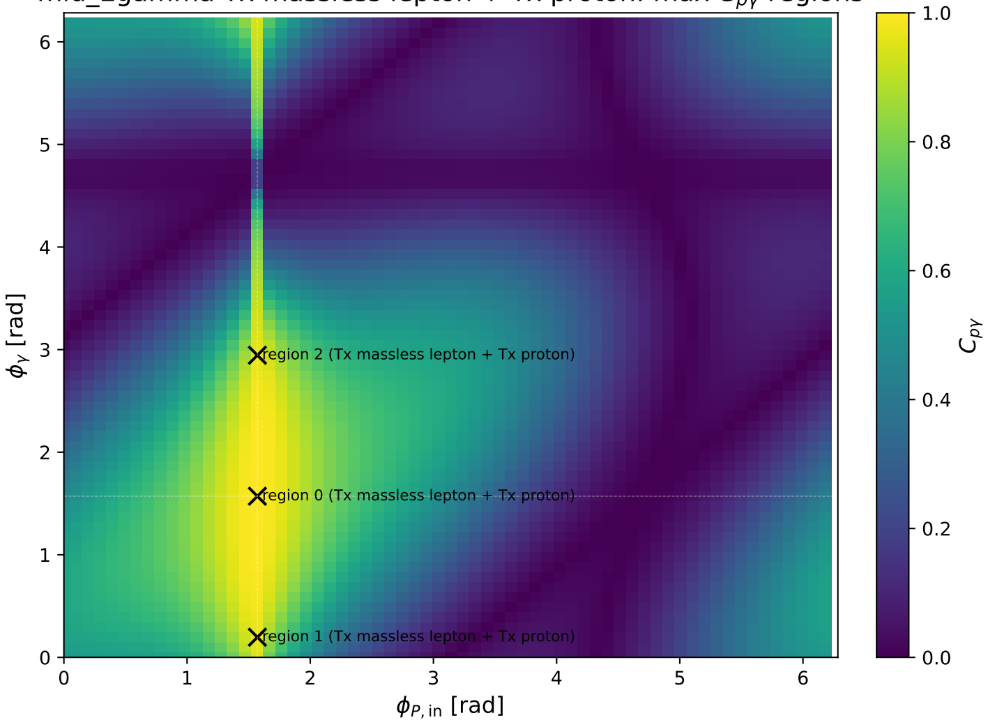
mid_Egamma Tx massless lepton + Tx proton: max C_{p\gamma} regions
