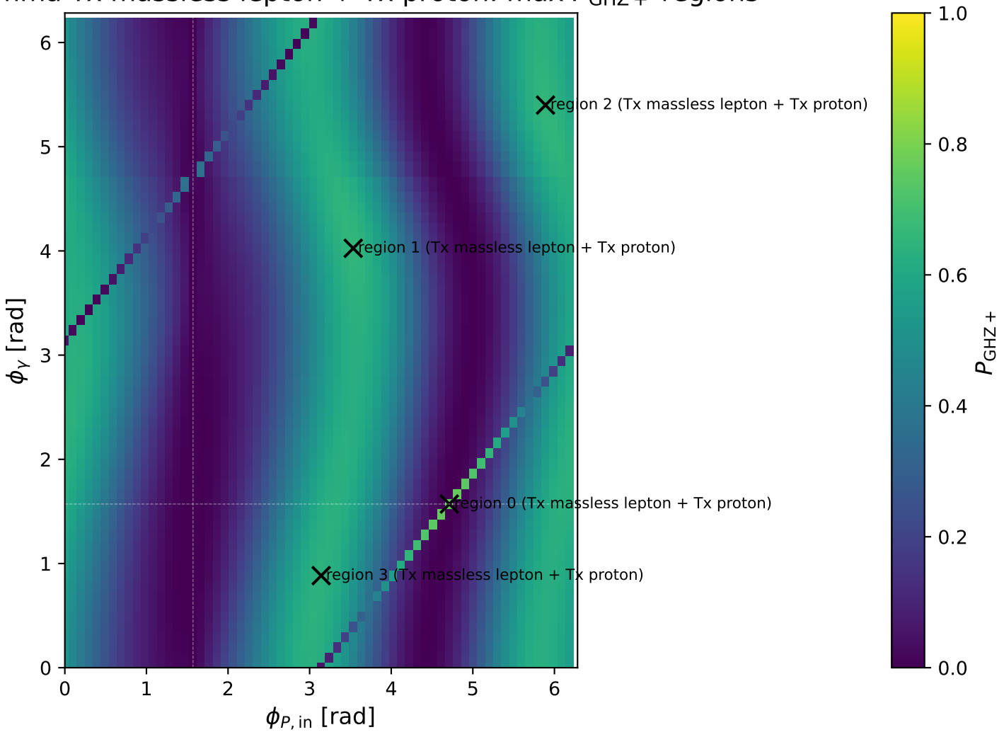
mma Tx massless lepton + Tx proton: max P_{\text{GHZ}+} regions
