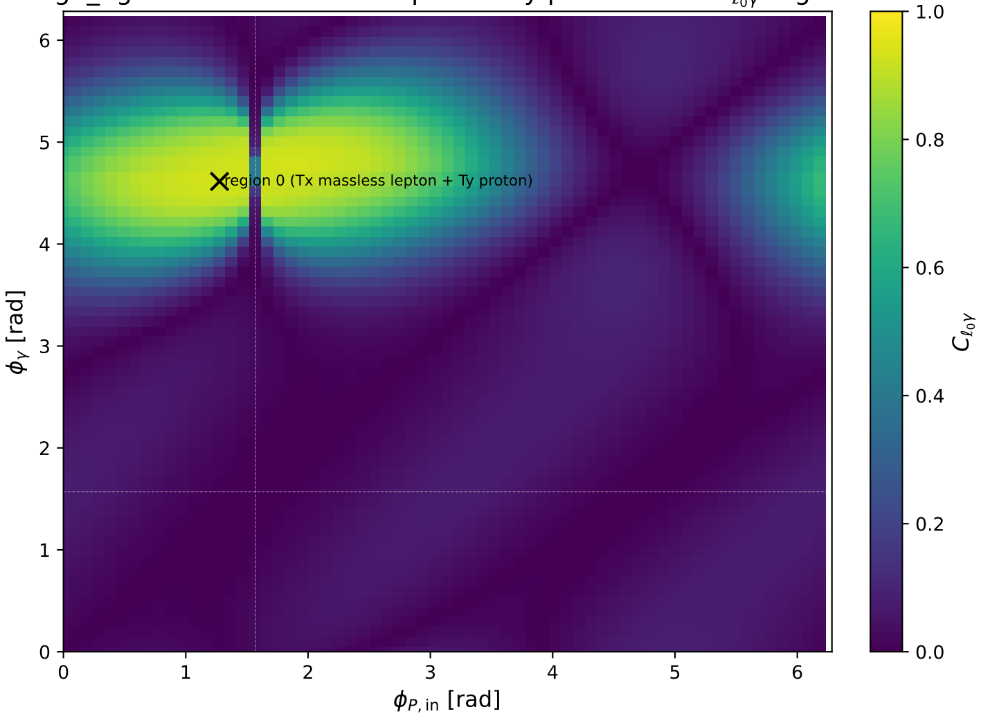
high_Egamma Tx massless lepton + Ty proton: max C_{\ell_0\gamma} regions
