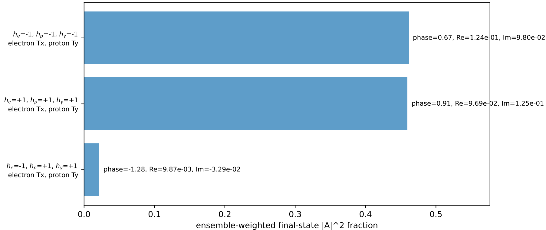
Leading initial-ensemble/final-state components (N=3, retained=94.3%)
