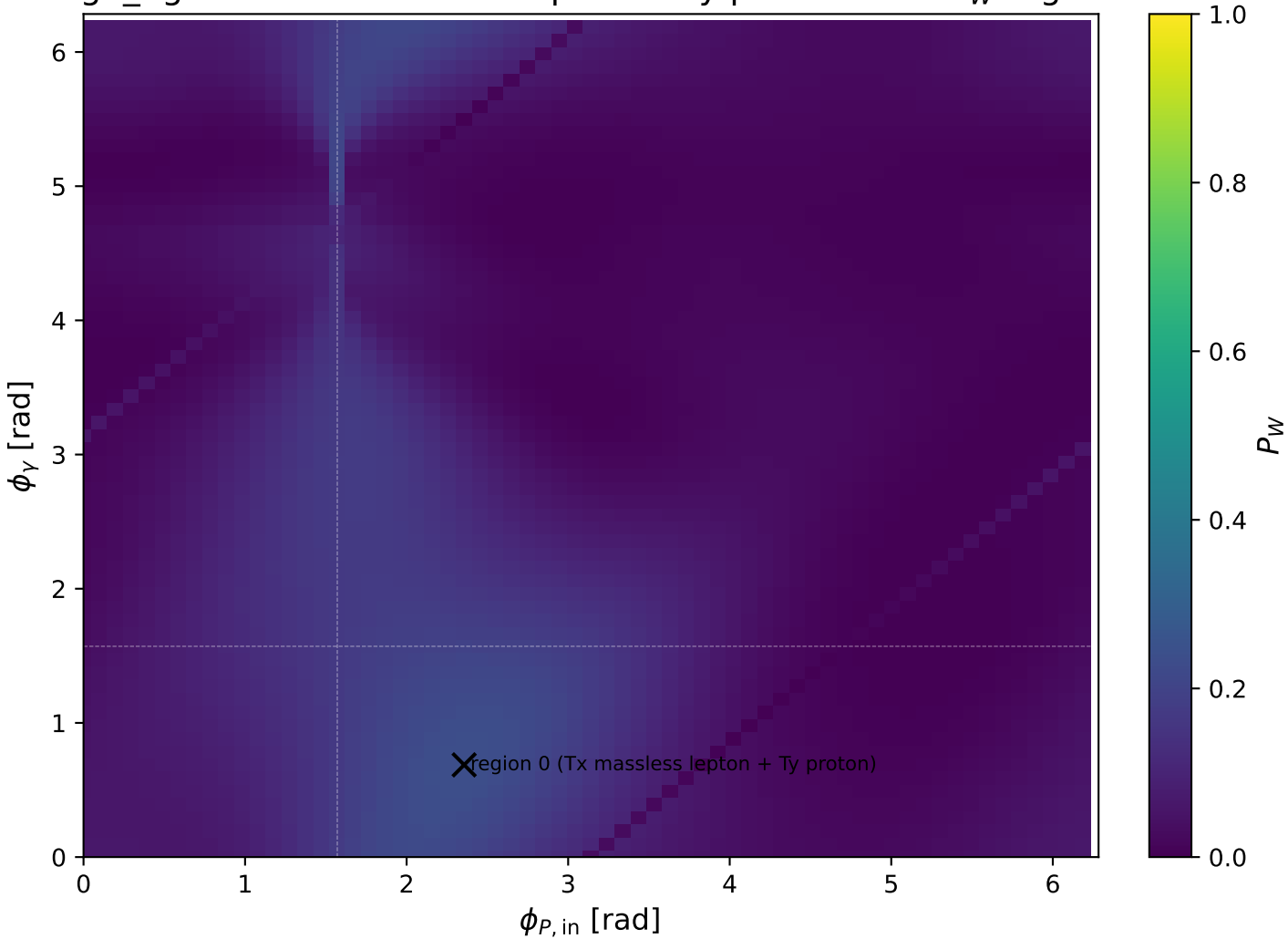
high_Egamma Tx massless lepton + Ty proton: max P_W regions
