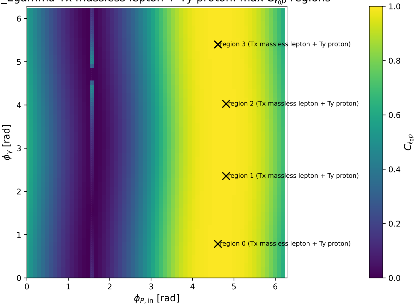
\gamma _Egamma Tx massless lepton + Ty proton: max C_{l_0p} regions
