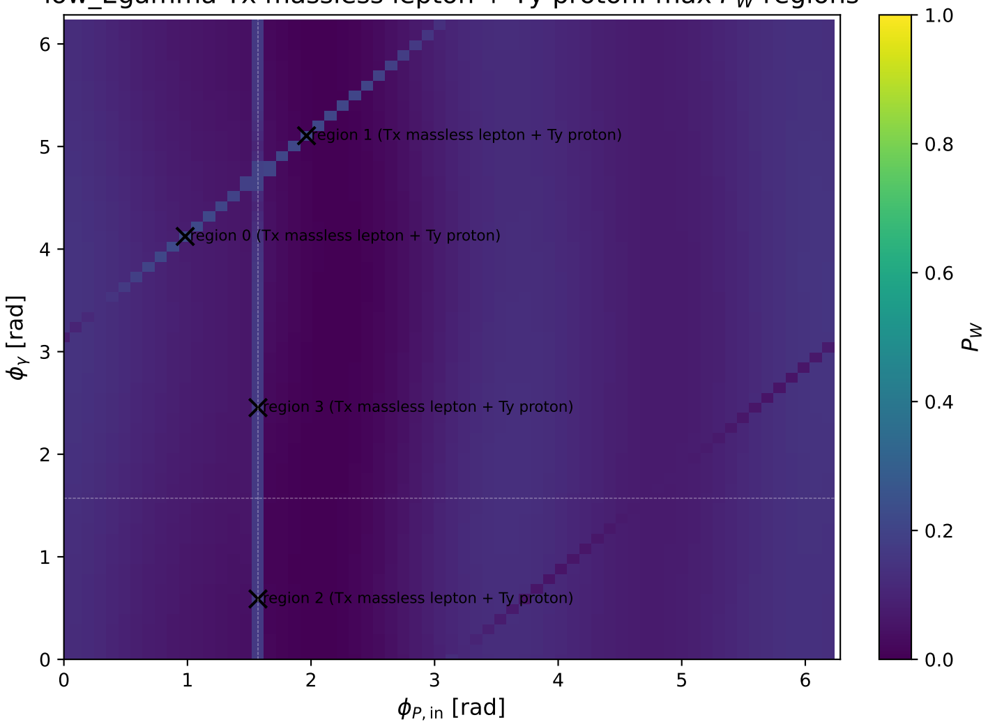
low_Egamma Tx massless lepton + Ty proton: max P_W regions
