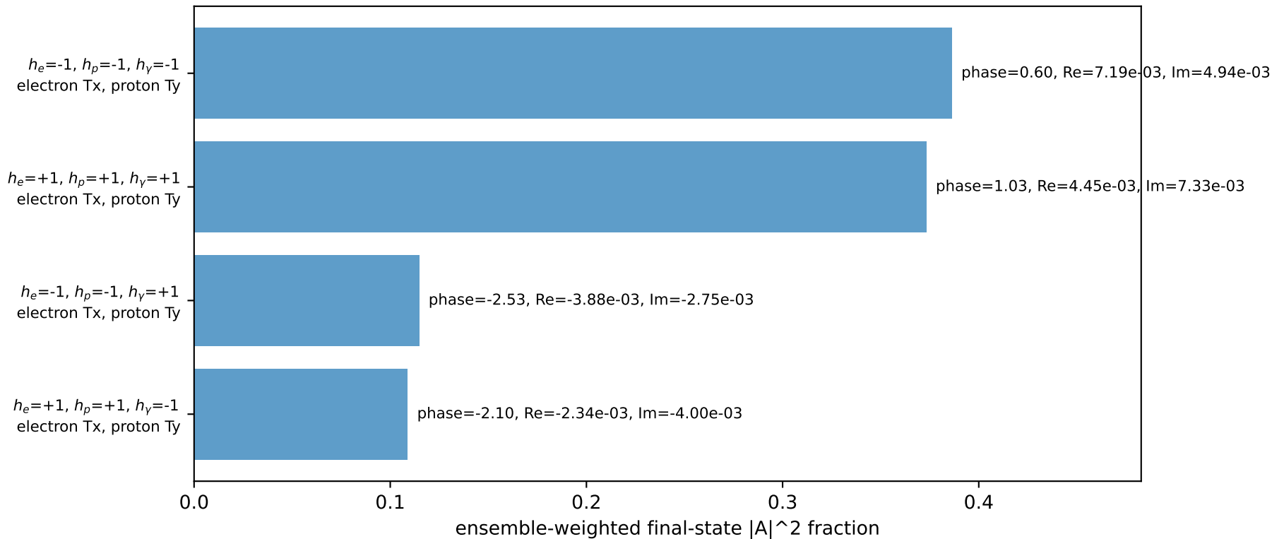
Leading initial-ensemble/final-state components (N=4, retained=98.3%)
