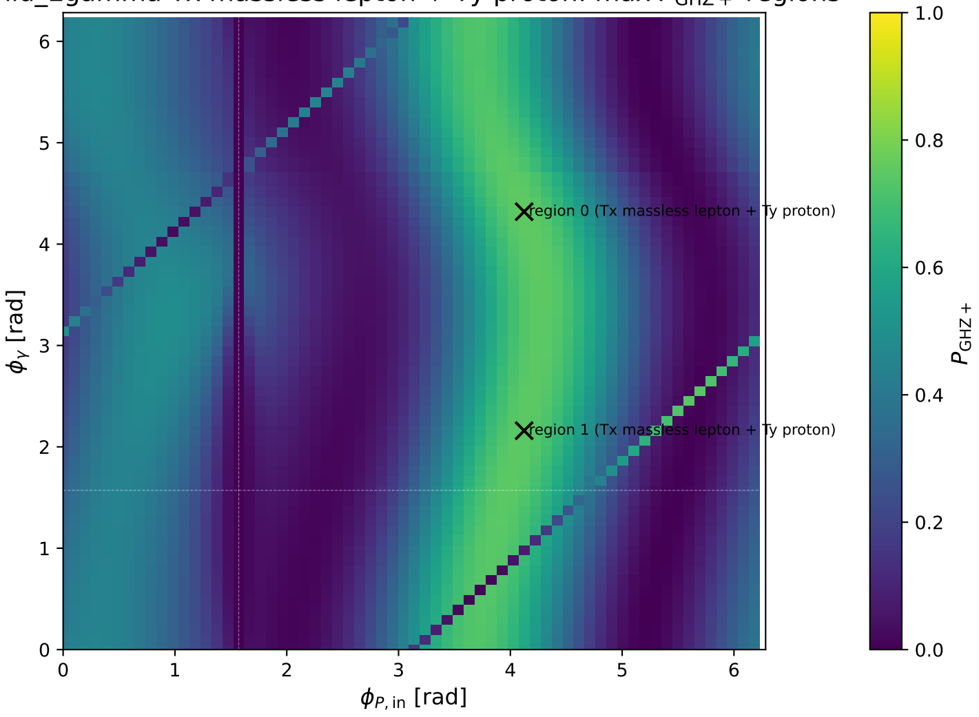
mid_Egamma Tx massless lepton + Ty proton: max P_{\text{GHz}} + regions
