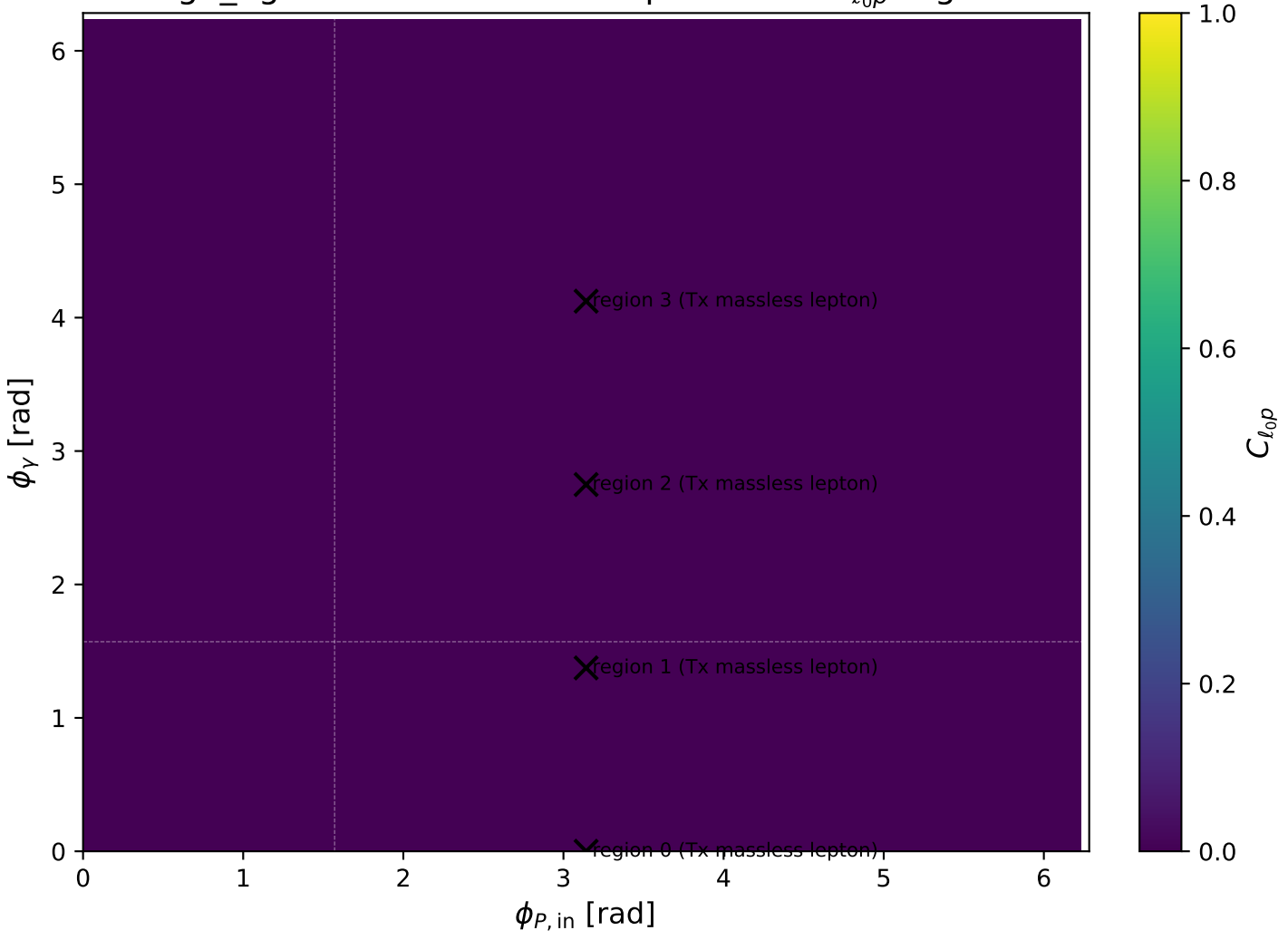
high_Egamma Tx massless lepton: max C_{\ell_0 p} regions
